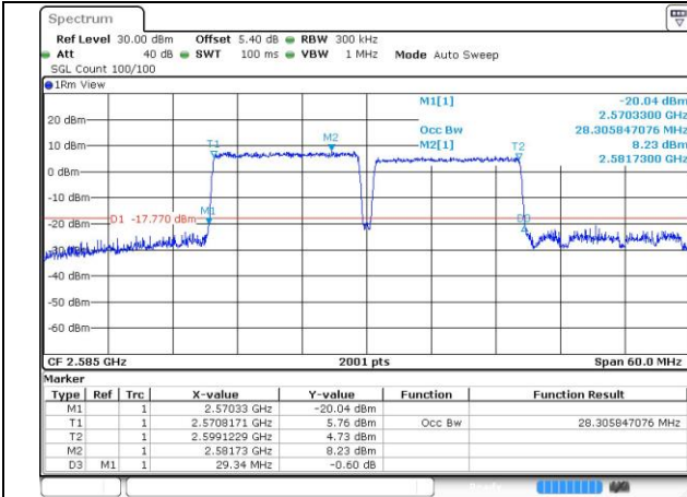
38-38-15MHz-15MHz-QPSK-QPSK-37825-37975-75R B#0-75RB#0
