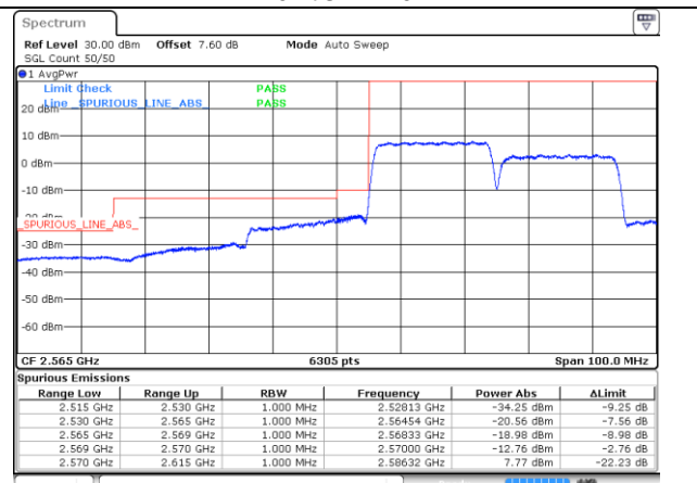
CA_38C_100RB+100RB_QPSK_37850+38048_100RB#0+100RB#0
