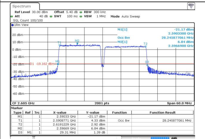
38-38-15MHz-15MHz-16QAM-16QAM-38025-38175- 75RB#0-75RB#0
