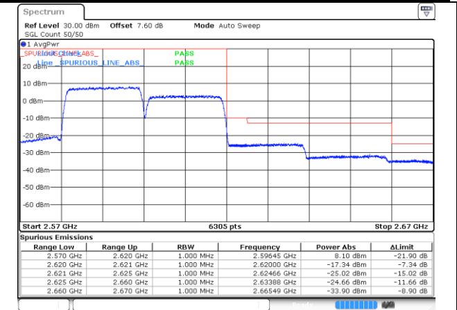
CA_38C_100RB+100RB_QPSK_37952+38150_100 RB#0+100RB#0
