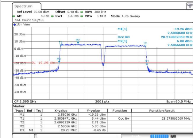
38-38-15MHz-15MHz-16QAM-16QAM-37925-38075- 75RB#0-75RB#0
