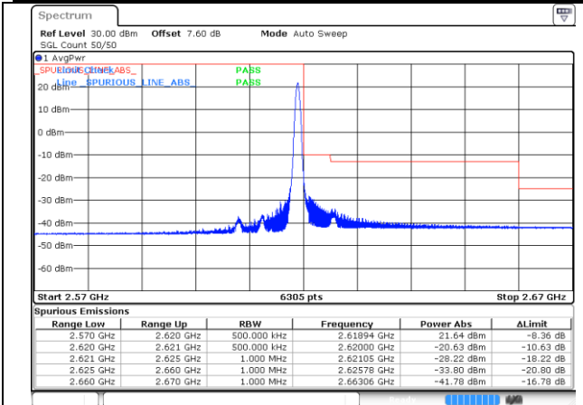
CA_38C_100RB+100RB_QPSK_37952+38150_0R B#0+1RB#99
