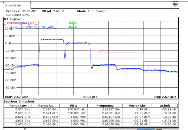
CA_38C_75RB+75RB_QPSK_37825+37975_75RB#0+75RB#0
