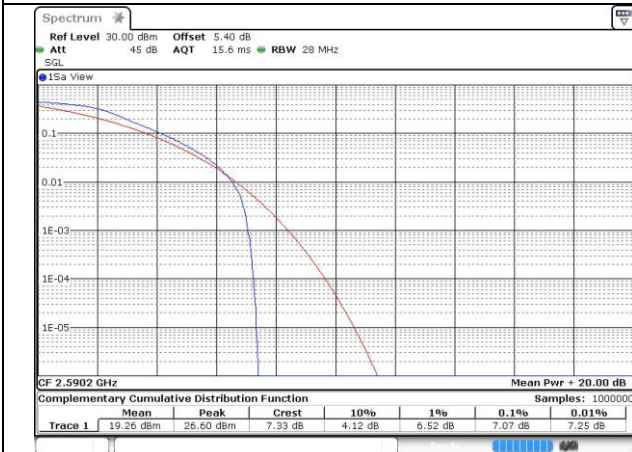
CA_38C_100RB+100RB_QPSK_37952+38150_100 RB#0+100RB#0
