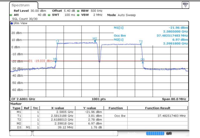
38-38-20MHz-20MHz-16QAM-16QAM-37952-38150-100RB#0-100RB#0
