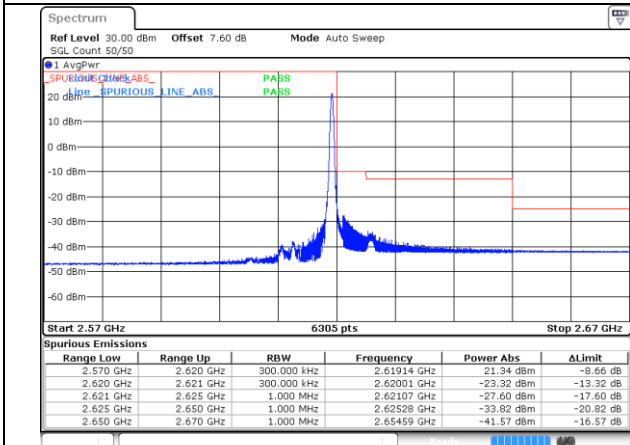
CA_38C_75RB+75RB_QPSK_37825+37975_1RB#0+0RB#0
