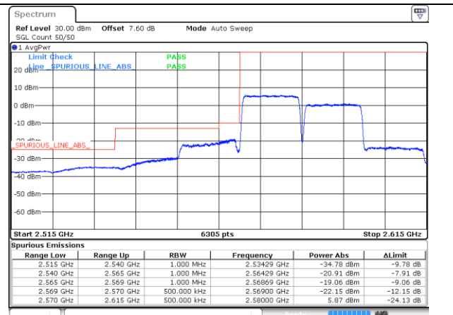
CA_38C_75RB+75RB_QPSK_37825+37975_75RB#0+75RB#0
