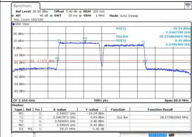
7-7-15MHz-15MHz-16QAM-16QAM-20825-20975-75 RB#0-75RB#0
