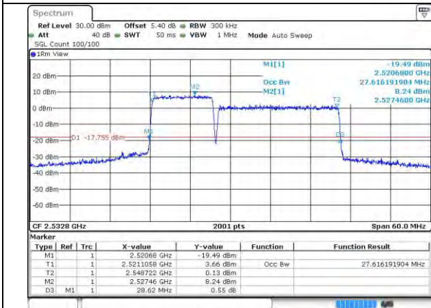
7-7-10MHz-20MHz-64QAM-64QAM-21206-21350-50 RB#0-100RB#0
