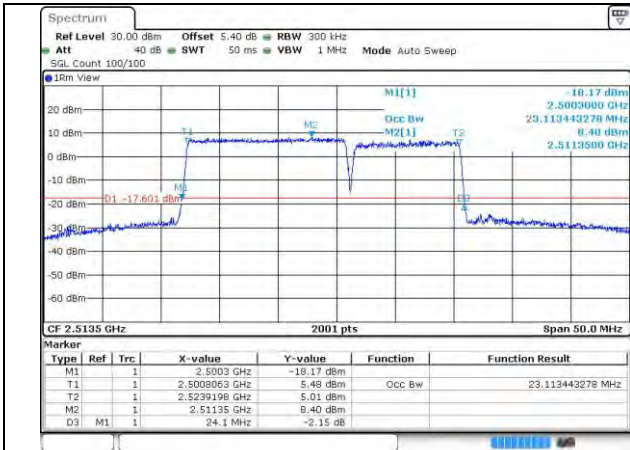
7-7-15MHz-10MHz-64QAM-64QAM-20825-20945-75 RB#0-50RB#0
