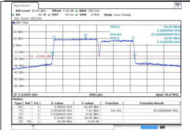
7-7-20MHz-15MHz-QPSK-QPSK-20850-21021-100R B#0-75RB#0
