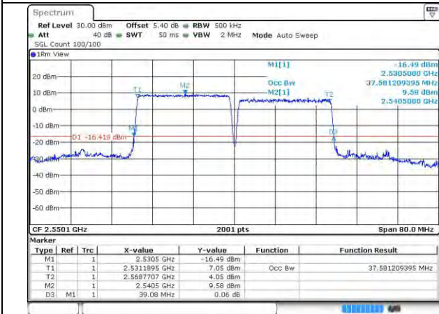
7-7-20MHz-20MHz-QPSK-QPSK-21152-21350-100RB #0-100RB#0
