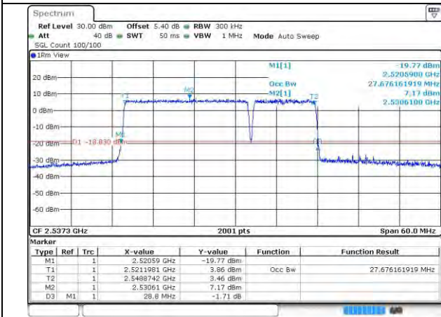
7-7-20MHz-10MHz-QPSK-QPSK-21251-21395-100R B#0-50RB#0
