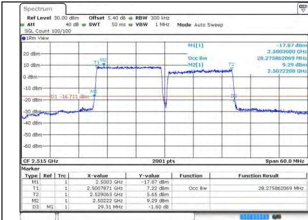
7-7-15MHz-15MHz-QPSK-QPSK-20825-20975-75RB #0-75RB#0
