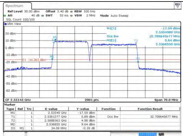
7-7-15MHz-20MHz-16QAM-16QAM-20828-20999 -75RB#0-100RB#0
