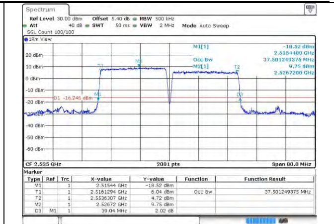
7-7-20MHz-20MHz-QPSK-QPSK-21001-21199-100RB #0-100RB#0
