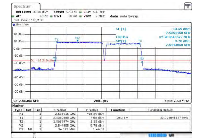
7-7-20MHz-15MHz-QPSK-QPSK-21201-21372-100R B#0-75RB#0
