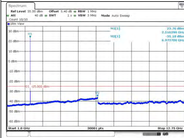
7-7-20MHz-20MHz-QPSK-QPSK-21001-21199 -1RB#0-0RB#0-1000~12750MHz
