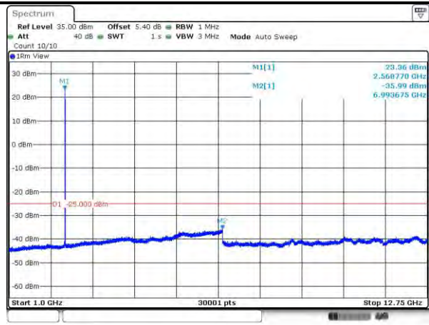
7-7-20MHz-20MHz-QPSK-QPSK-21152-21350 -ORB#0-1RB#99-1000~12750MHz
