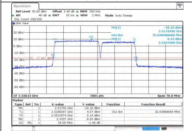
7-7-20MHz-15MHz-16QAM-16QAM-21026-21197-10 ORB#0-75RB#0
