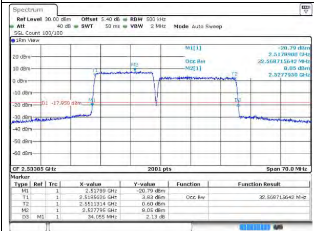
7-7-15MHz-20MHz-64QAM-64QAM-21179-21350 -75RB#0-100RB#0
