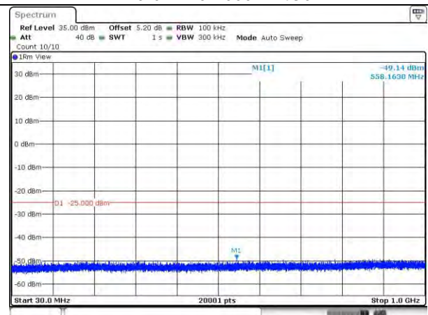
7-7-20MHz-20MHz-QPSK-QPSK-21001-21199 -ORB#0-1RB#99-30~1000MHz
