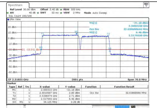
7-7-20MHz-15MHz-256QAM-256QAM-20850-21021- 100RB#0-75RB#0
