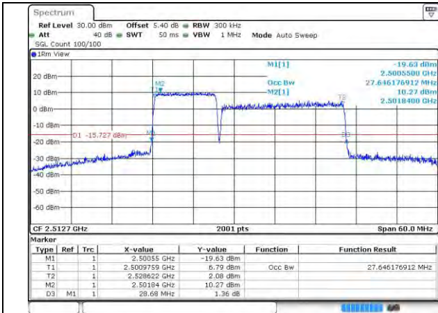
7-7-10MHz-20MHz-64QAM-64QAM-20805-20949-50 RB#0-100RB#0
