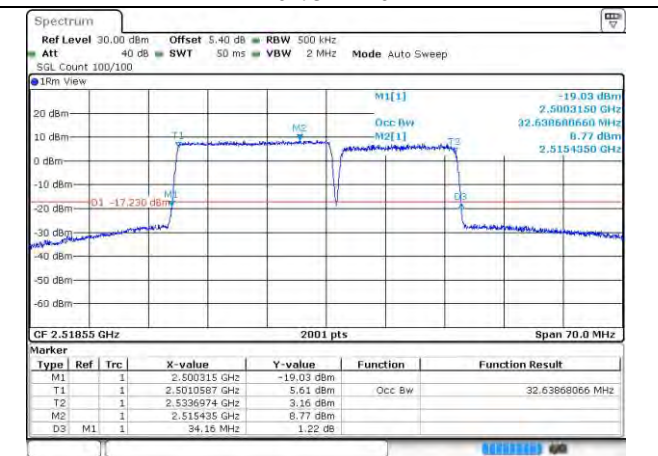
7-7-20MHz-15MHz-16QAM-16QAM-20850-21021-10 ORB#0-75RB#0
