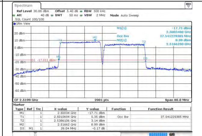
7-7-20MHz-20MHz-16QAM-16QAM-20850-21048-10 ORB#0-100RB#0
