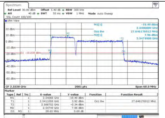
7-7-10MHz-20MHz-256QAM-256QAM-20805-20949-50RB#0-100RB#0
