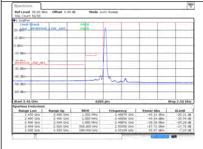
CA_7C_100RB+100RB_QPSK_20850+21048_1RB#0 +0RB#0
