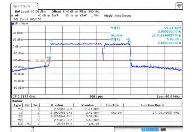
7-7-20MHz-10MHz-256QAM-256QAM-20850-20994- 100RB#0-50RB#0
