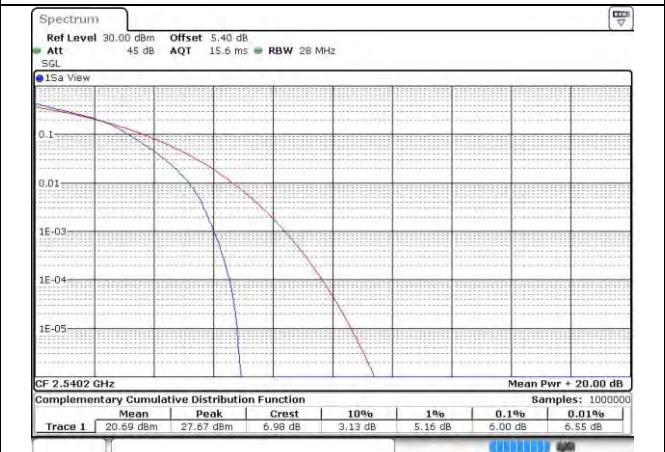
CA_7C_100RB+100RB_16QAM_21048+20850_100RB#0+100RB#0
