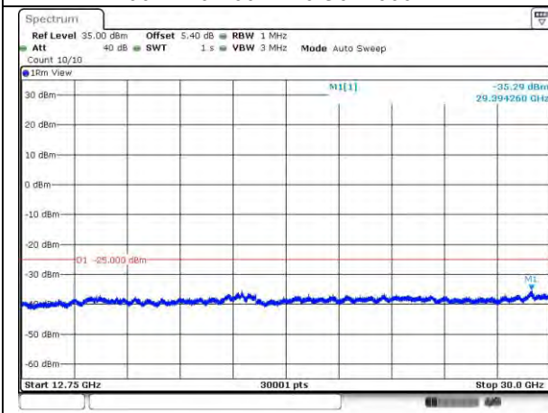
7-7-20MHz-20MHz-QPSK-QPSK-21001-21199 -100RB#0-100RB#0-12750~30000MHz
