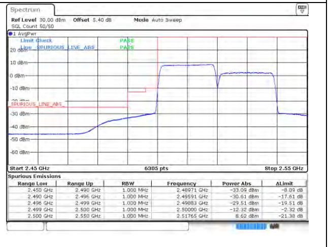
CA_7C_100RB+100RB_QPSK_20850+21048_100RB#0 +100RB#0
