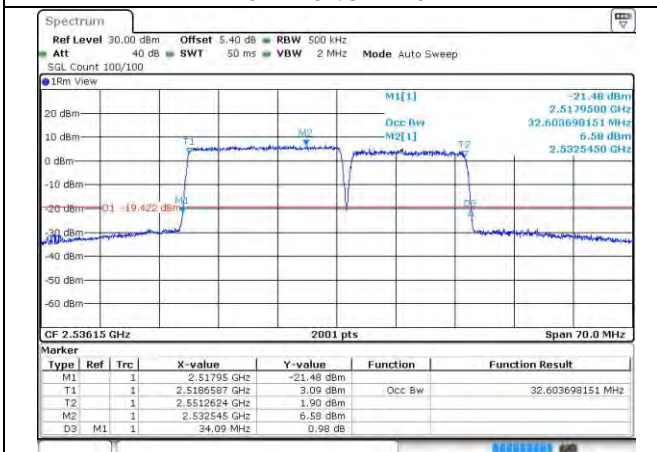
7-7-20MHz-15MHz-256QAM-256QAM-21026-21197- 100RB#0-75RB#0
