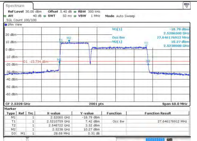
7-7-10MHz-20MHz-64QAM-64QAM-21006-21150-50 RB#0-100RB#0
