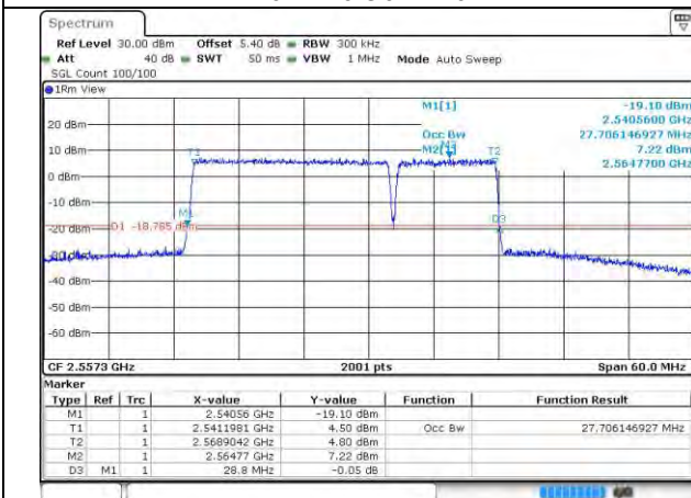
7-7-20MHz-10MHz-64QAM-64QAM-21251-21395-10 ORB#0-50RB#0
