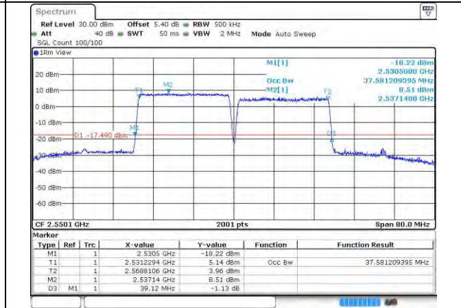
7-7-20MHz-20MHz-16QAM-16QAM-21152-21350-10 ORB#0-100RB#0
