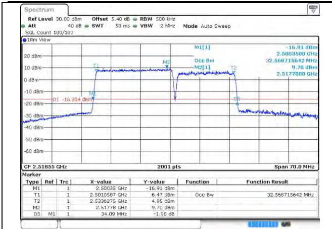
7-7-20MHz-15MHz-64QAM-64QAM-20850-21021-10 ORB#0-75RB#0
