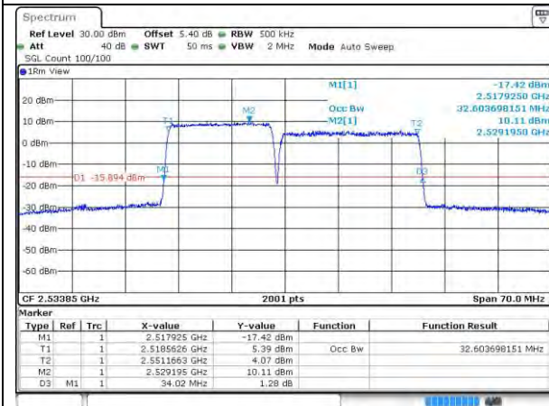
7-7-15MHz-20MHz-QPSK-QPSK-21179-21350-75 RB#0-100RB#0
