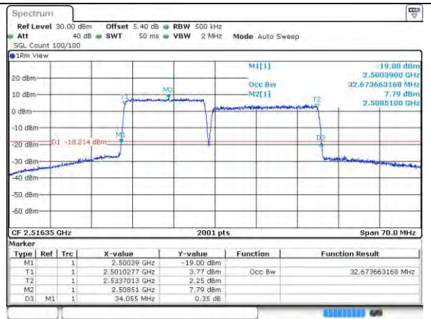
7-7-15MHz-20MHz-64QAM-64QAM-21003-21174 -75RB#0-100RB#0
