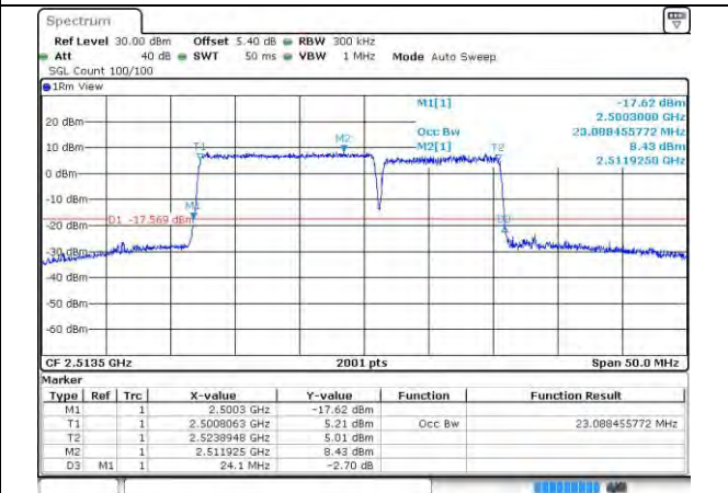
7-7-15MHz-10MHz-QPSK-QPSK-21051-21171-75RB# 0-50RB#0
