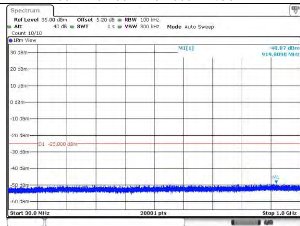
7-7-20MHz-20MHz-QPSK-QPSK-21001-21199 -1RB#0-0RB#0-30~1000MHz
