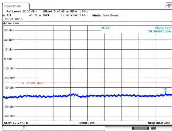
7-7-20MHz-20MHz-QPSK-QPSK-21152-21350 -100RB#0-100RB#0-12750~30000MHz
