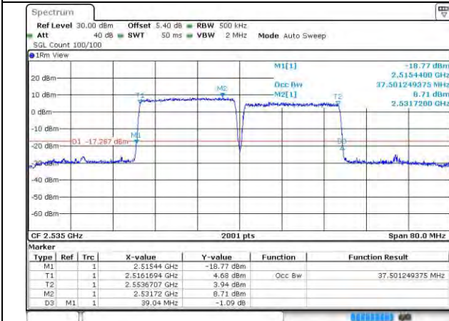
7-7-20MHz-20MHz-16QAM-16QAM-21001-21199-10 ORB#0-100RB#0
