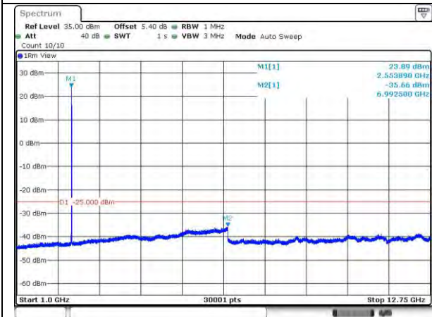
7-7-20MHz-20MHz-QPSK-QPSK-21001-21199 -ORB#0-1RB#99-1000~12750MHz
