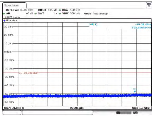
7-7-20MHz-20MHz-QPSK-QPSK-21152-21350 -100RB#0-100RB#0-30~1000MHz
