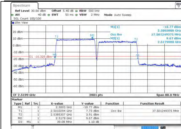
7-7-20MHz-20MHz-QPSK-QPSK-20850-21048-100R B#0-100RB#0
