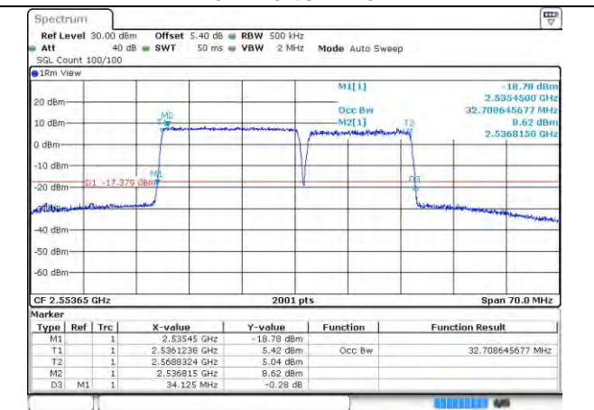
7-7-20MHz-15MHz-16QAM-16QAM-21201-21372-10 ORB#0-75RB#0
