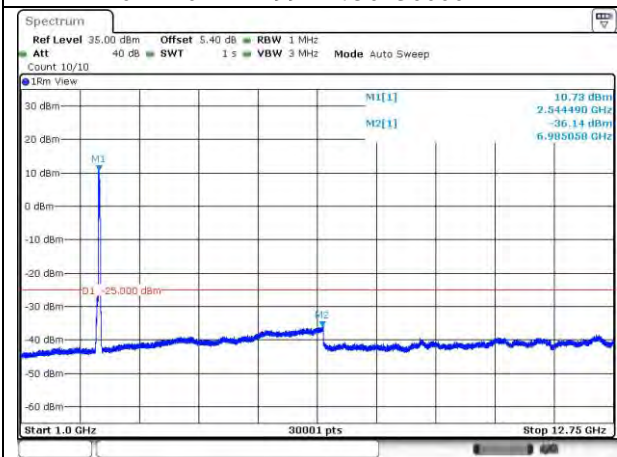
7-7-20MHz-20MHz-QPSK-QPSK-21152-21350 -100RB#0-100RB#0-1000~12750MHz
