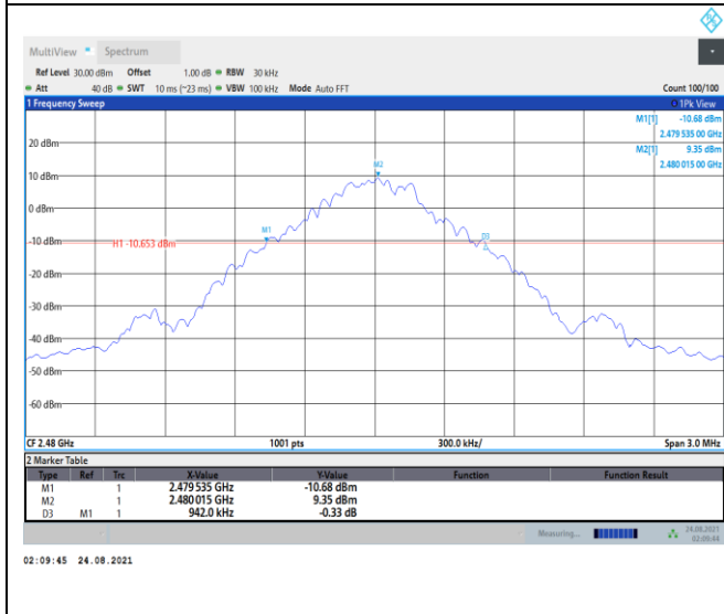
Modulation: GFSK 2480MHz
