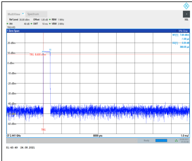
Modulation: GFSK DH1 2441
