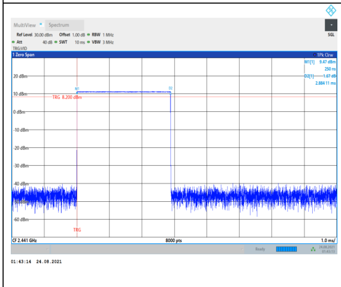
Modulation: GFSK DH5 2441
