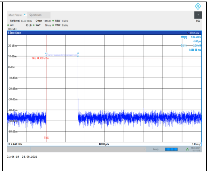
Modulation: GFSK DH3 2441
