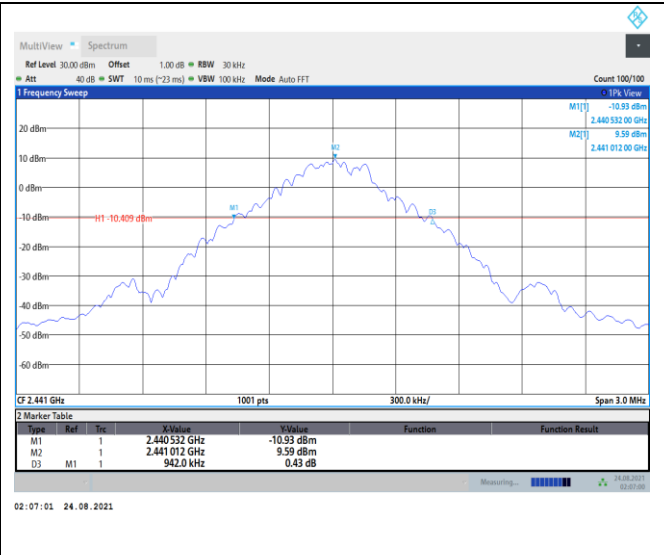
Modulation: GFSK 2441MHz
