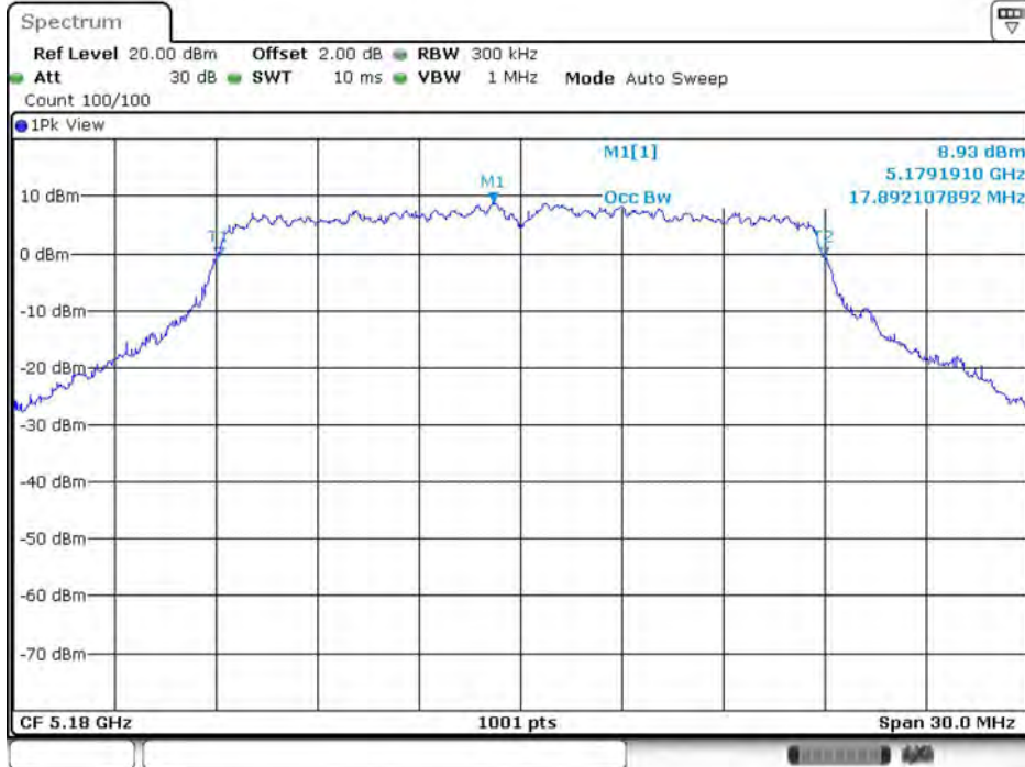
11AC20SISO_Ant9_5180
