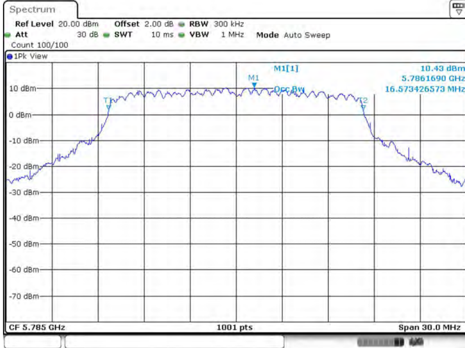
11A-CDD_Ant10_5785
