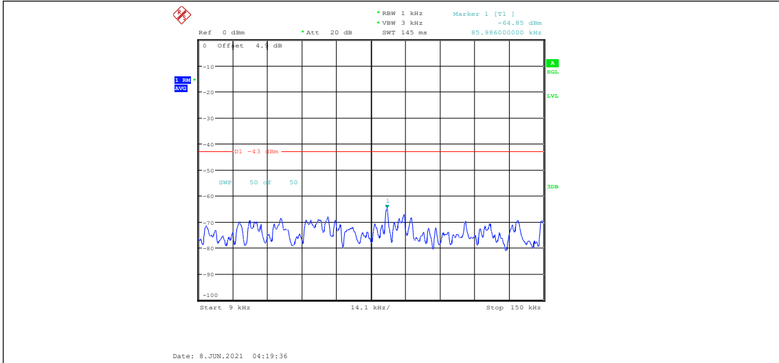
NTNV-DC_5A_n2A-15kHz-5MHz+20MHz-N/A+DFT-PI2BPSK-Mid+High-N/A-Edge_1RB_Left -0.009-0.15-----43-PASS
