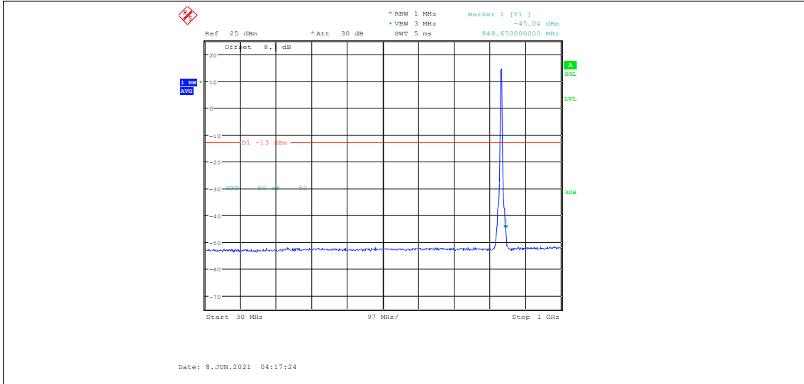
NTNV-DC_5A_n2A-15kHz-5MHz+20MHz-N/A+DFT-PI2BPSK-Mid+Low-N/A-Edge_1RB_Left-30-1000-----13-PASS
