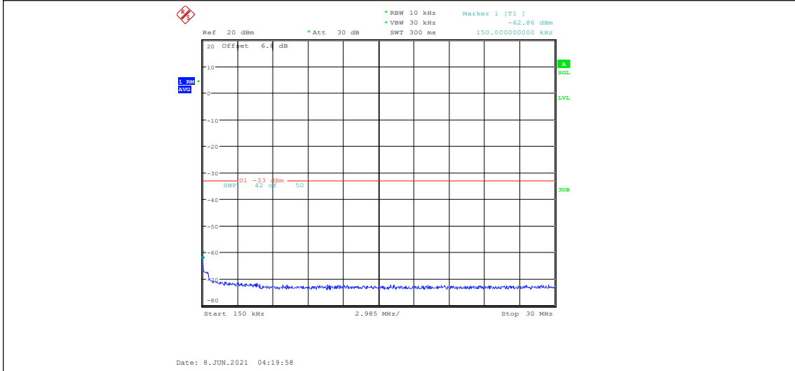
NTNV-DC_5A_n2A-15kHz-5MHz+20MHz-N/A+DFT-PI2BPSK-Mid+High-N/A-Edge_1RB_Left -0.15-30-----33-PASS
