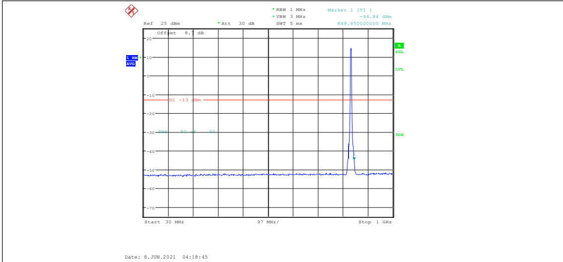
NTNV-DC_5A_n2A-15kHz-5MHz+20MHz-N/A+DFT-PI2BPSK-Mid+Mid-N/A-Edge_1RB_Left-30-1000-----13-PASS
