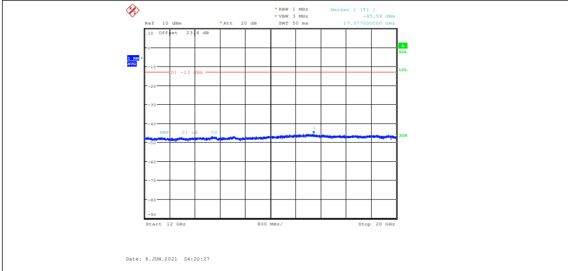
NTNV-DC_5A_n2A-15kHz-5MHz+20MHz-N/A+DFT-PI2BPSK-Mid+High-N/A-Edge_1RB_Left -12000-20000-----13-PASS
