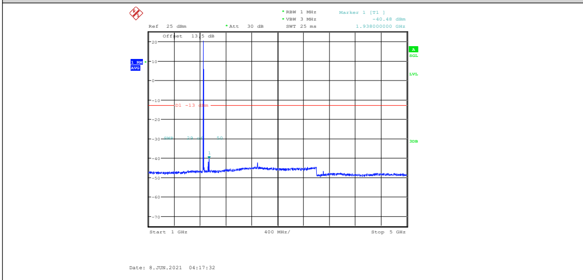
NTNV-DC_5A_n2A-15kHz-5MHz+20MHz-N/A+DFT-PI2BPSK-Mid+Low-N/A-Edge_1RB_Left-1000-5000-----13-PASS
