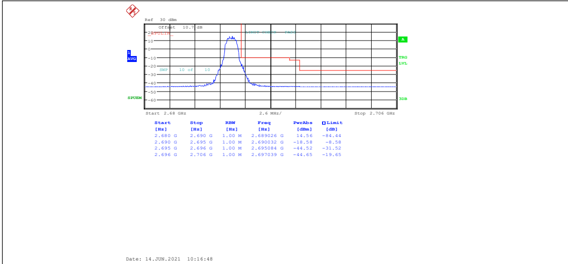
NTNV-DC_2A_n41A-30kHz-5MHz+100MHz-N/A+CP-QPSK-Mid+High-N/A-Edge_1RB_Right -----see graph-PASS
