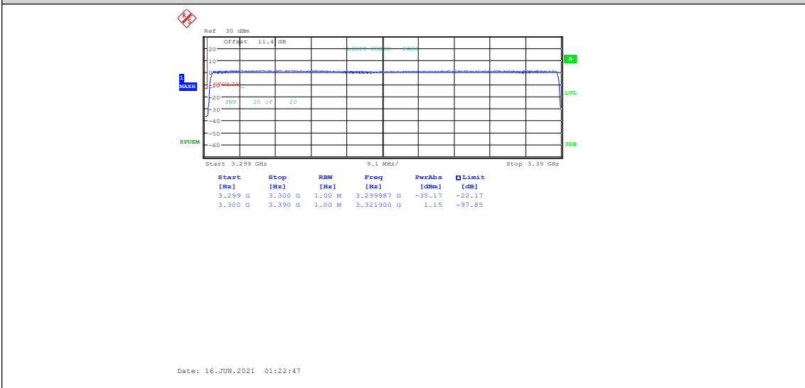
NTNV-DC_5A_n77A-30kHz-5MHz+90MHz-N/A+CP-QPSK-Mid+Low-N/A-Outer_Full----- -see graph-PASS
