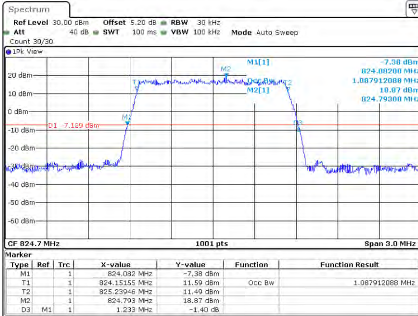
Band26-1.4MHz-QPSK-26797-6RB#0-1.088
