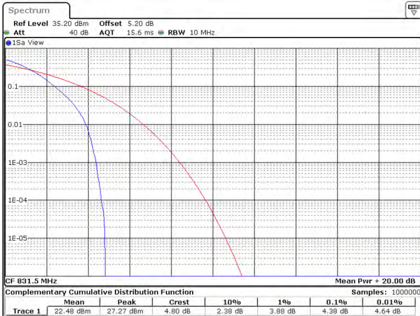
Band26-15MHz-QPSK-26865-75RB#0
