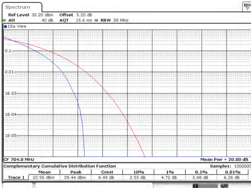
Band12-10MHz-QPSK-23060-50RB#0
