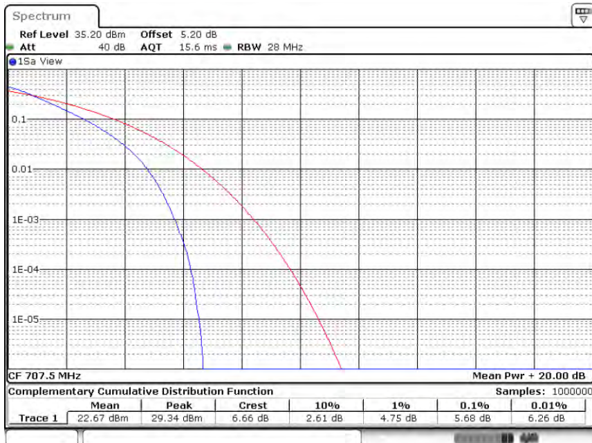
Band12-10MHz-QPSK-23095-50RB#0
