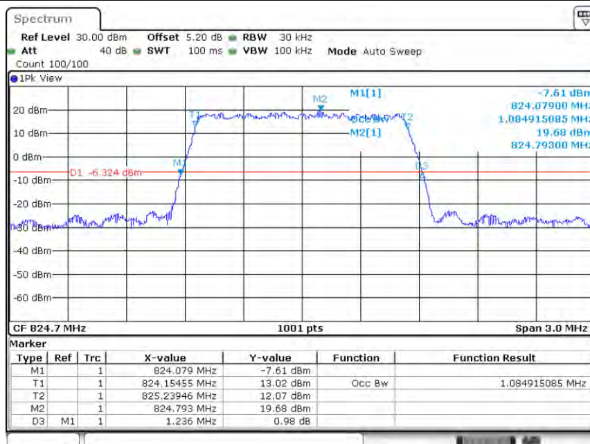
Band5-1.4MHz-QPSK-20407-6RB#0-1.085
