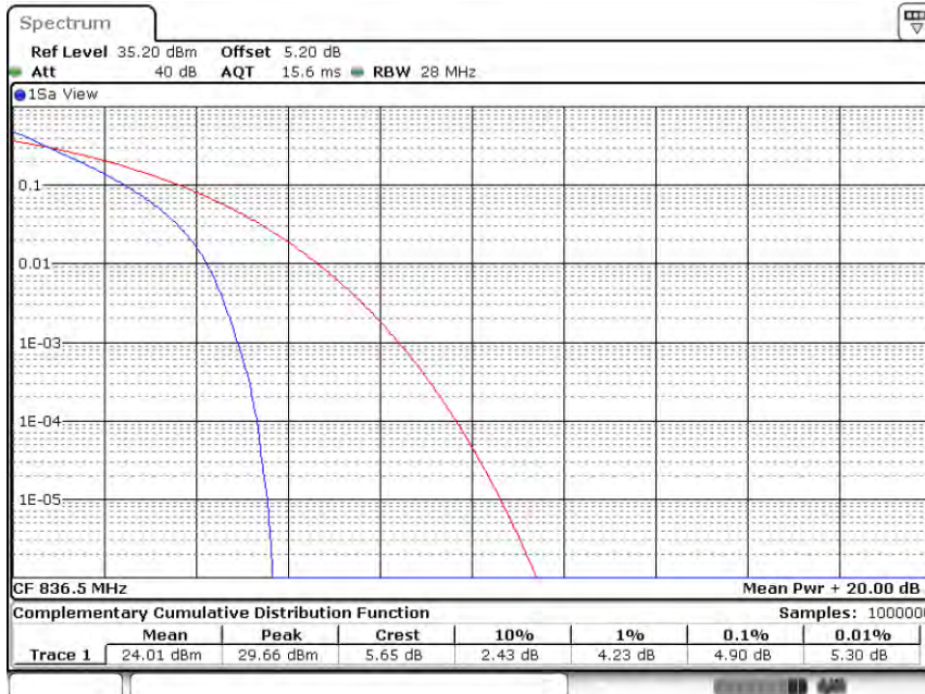
Band5-10MHz-QPSK-20525-50RB#0
