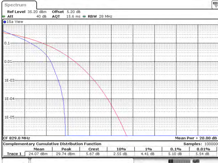
Band5-10MHz-QPSK-20450-50RB#0
