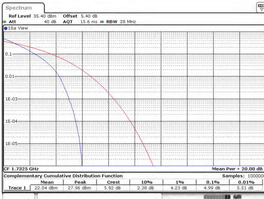
Band4-20MHz-QPSK-20175-100RB#0
