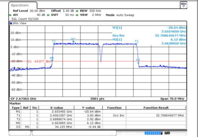
41-41-20MHz-15MHz-256QAM-256QAM-41341-41512-100RB#0-75RB#0
