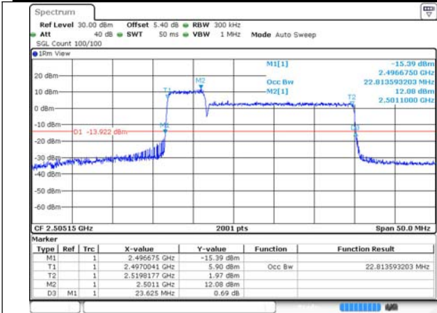
41-41-5MHz-20MHz-64QAM-64QAM-39683-39800-2 5RB#0-100RB#0
