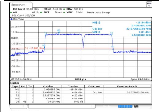
41-41-20MHz-15MHz-64QAM-64QAM-39750-39921-100RB#0-75RB#0
