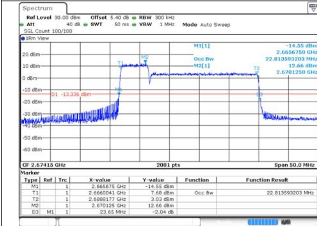
41-41-5MHz-20MHz-64QAM-64QAM-41373-41490-2 5RB#0-100RB#0
