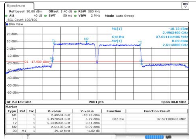
41-41-20MHz-20MHz-16QAM-16QAM-39750-39948-100RB#0-100RB#0
