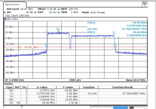
41-41-10MHz-20MHz-QPSK-QPSK-40526-40670-50R B#0-100RB#0
