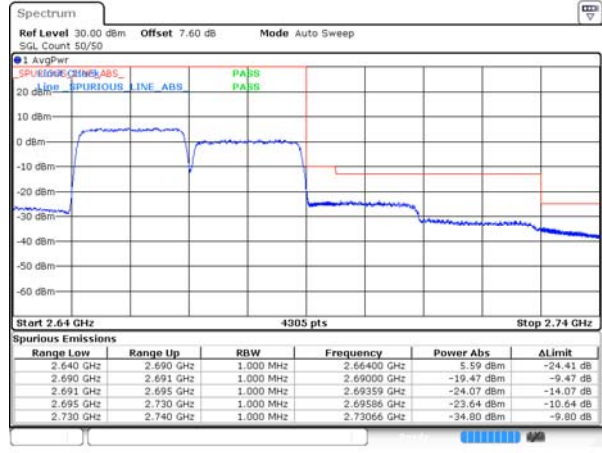
CA_41C_100RB+100RB_QPSK_41292+41490_100 RB#0+100RB#0
