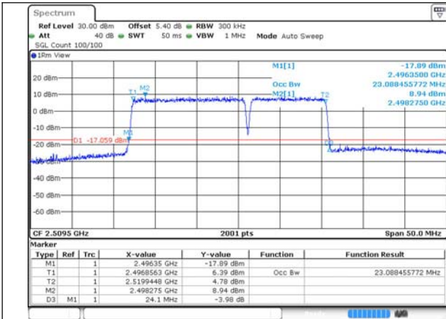
41-41-15MHz-10MHz-QPSK-QPSK-39725-39845-75R B#0-50RB#0
