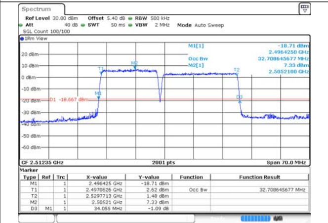
41-41-15MHz-20MHz-256QAM-256QAM-39728-3989-9-75RB#0-100RB#0
