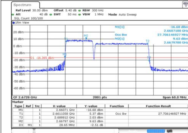
41-41-10MHz-20MHz-64QAM-64QAM-41346-41490-50RB#0-100RB#0
