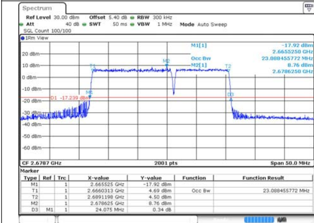
41-41-15MHz-10MHz-64QAM-64QAM-41417-41537-75RB#0-50RB#0
