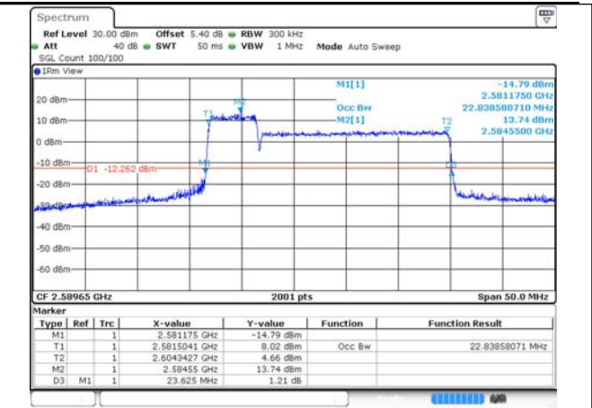
41-41-5MHz-20MHz-QPSK-QPSK-40528-40645-25R B#0-100RB#0
