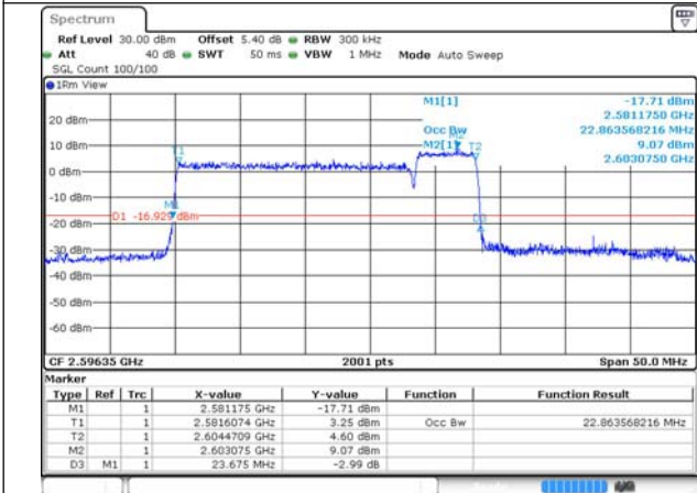
41-41-20MHz-5MHz-256QAM-256QAM-40595-40712-100RB#0-25RB#0
