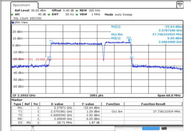
41-41-20MHz-10MHz-256QAM-256QAM-40571-40715-100RB#0-50RB#0
