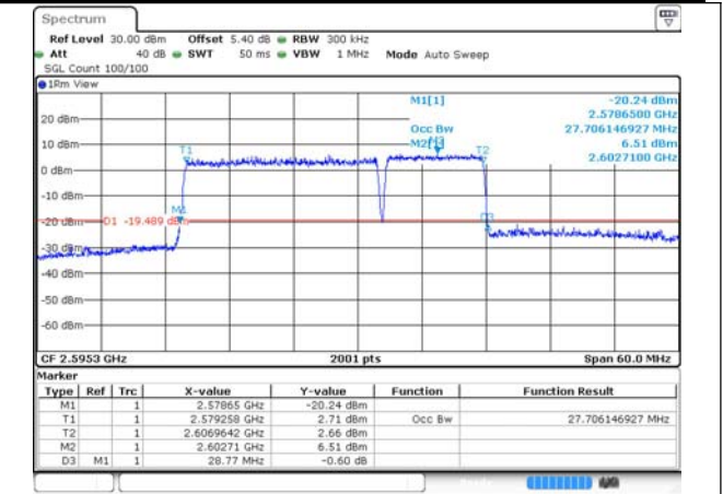
41-41-20MHz-10MHz-64QAM-64QAM-40571-40715-100RB#0-50RB#0
