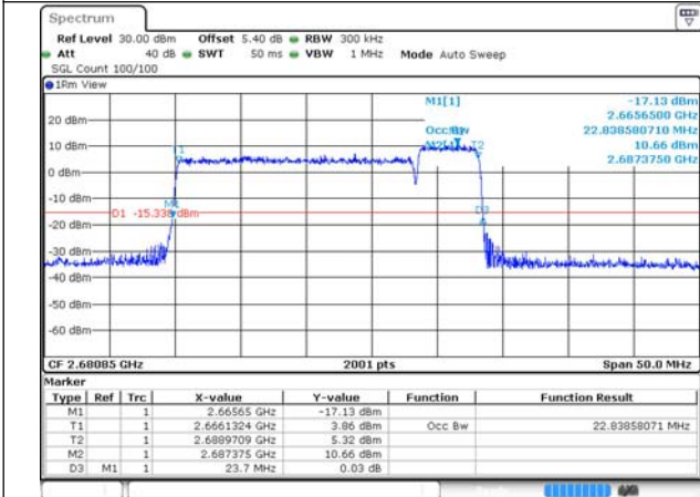
41-41-20MHz-5MHz-64QAM-64QAM-41440-41557-1 00RB#0-25RB#0
