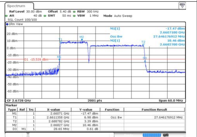
41-41-10MHz-20MHz-16QAM-16QAM-41346-41490-50RB#0-100RB#0
