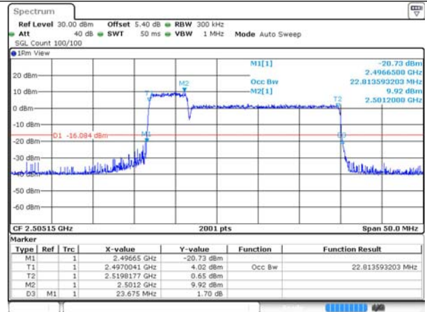
41-41-5MHz-20MHz-256QAM-256QAM-39683-39800 -25RB#0-100RB#0
