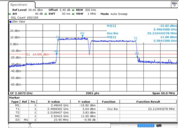
41-41-10MHz-15MHz-16QAM-16QAM-39703-39823-50RB#0-75RB#0
