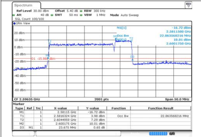
41-41-20MHz-5MHz-16QAM-16QAM-40595-40712-100RB#0-25RB#0
