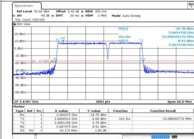
41-41-15MHz-10MHz-QPSK-QPSK-41417-41537-75R B#0-50RB#0
