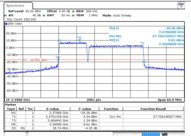
41-41-10MHz-20MHz-64QAM-64QAM-40526-40670-50RB#0-100RB#0
