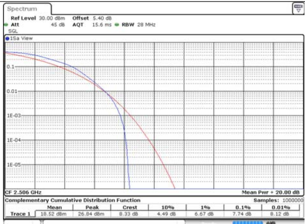
CA_41C_100RB+100RB_16QAM_41292+41490_100 RB#0+100RB#0
