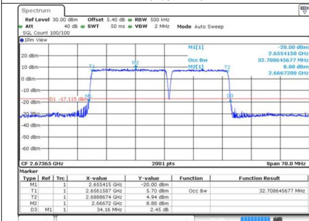
41-41-20MHz-15MHz-QPSK-QPSK-41341-41512-100 RB#0-75RB#0
