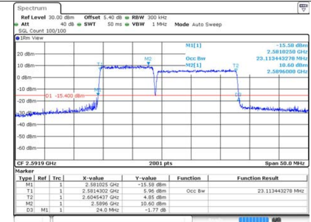
41-41-10MHz-15MHz-QPSK-QPSK-40549-40669-50R B#0-75RB#0
