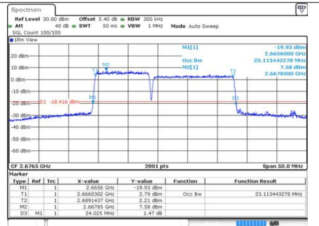
41-41-10MHz-15MHz-256QAM-256QAM-41395-41515-50RB#0-75RB#0
