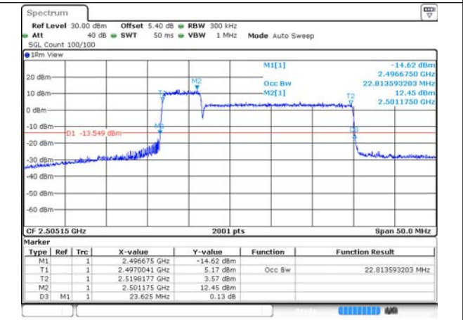
41-41-5MHz-20MHz-16QAM-16QAM-39683-39800-2 5RB#0-100RB#0
