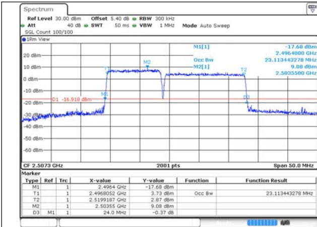
41-41-10MHz-15MHz-64QAM-64QAM-39703-39823-50RB#0-75RB#0
