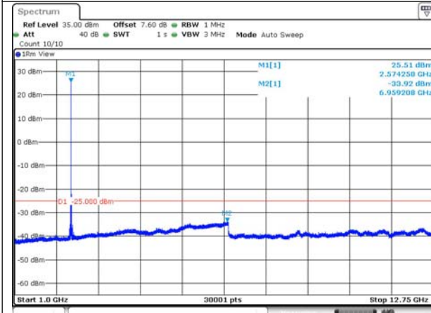
41-41-20MHz-20MHz-QPSK-QPSK-40521-40719 -1RB#0-0RB#0-1000~12750MHz
