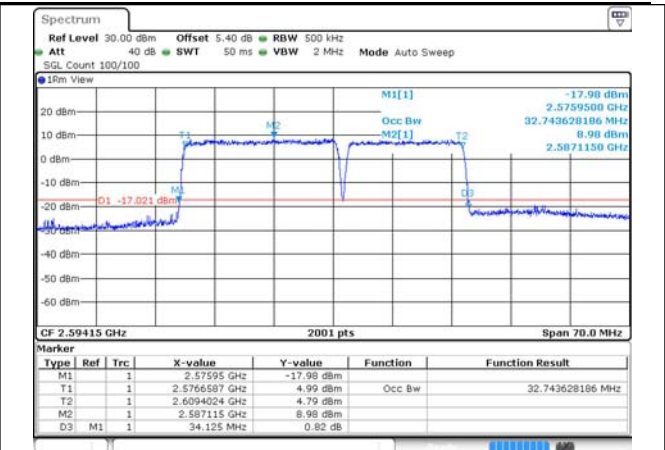
41-41-20MHz-15MHz-QPSK-QPSK-40546-40717-100 RB#0-75RB#0
