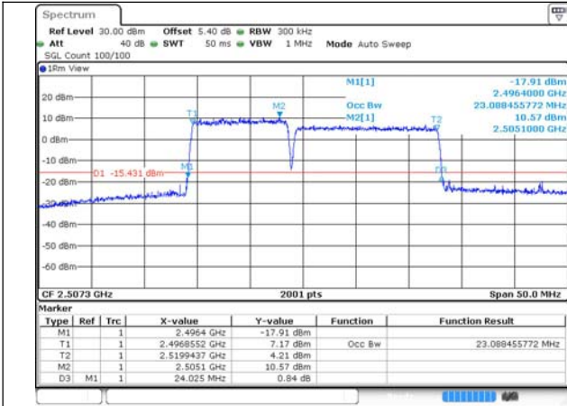
41-41-10MHz-15MHz-QPSK-QPSK-39703-39823-50R B#0-75RB#0
