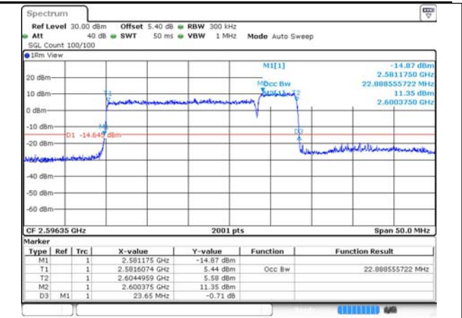
41-41-20MHz-5MHz-QPSK-QPSK-40595-40712-100R B#0-25RB#0
