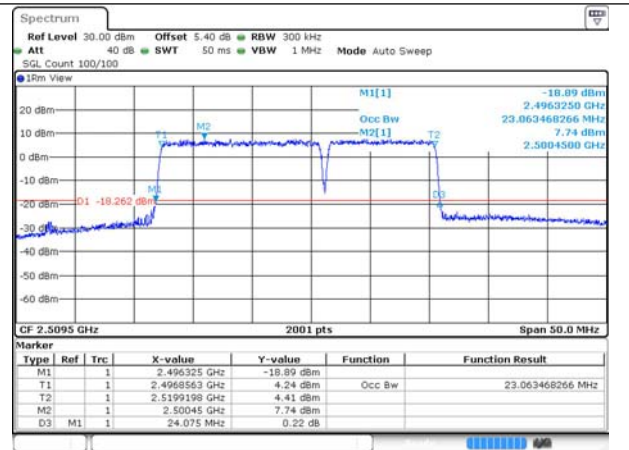
41-41-15MHz-10MHz-16QAM-16QAM-39725-39845-75RB#0-50RB#0
