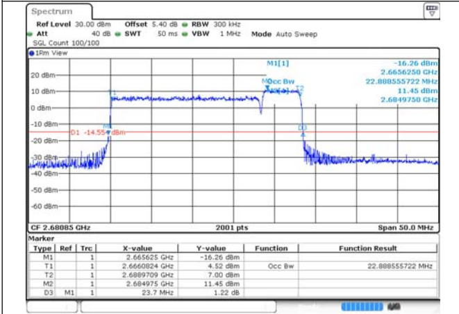
41-41-20MHz-5MHz-QPSK-QPSK-41440-41557-100R B#0-25RB#0
