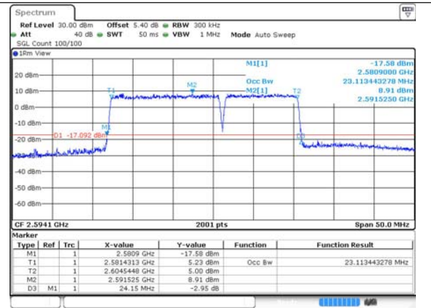
41-41-15MHz-10MHz-QPSK-QPSK-40571-40691-75R B#0-50RB#0
