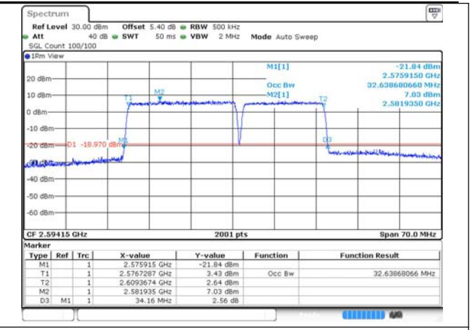
41-41-20MHz-15MHz-64QAM-64QAM-40546-40717-100RB#0-75RB#0
