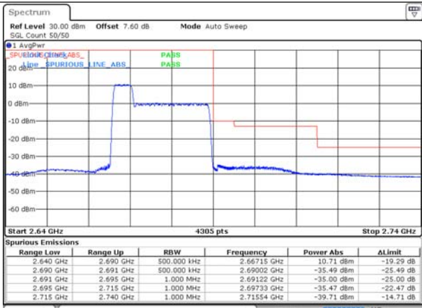
CA_41C_100RB+100RB_QPSK_39750+39948_100 RB#0+100RB#0
