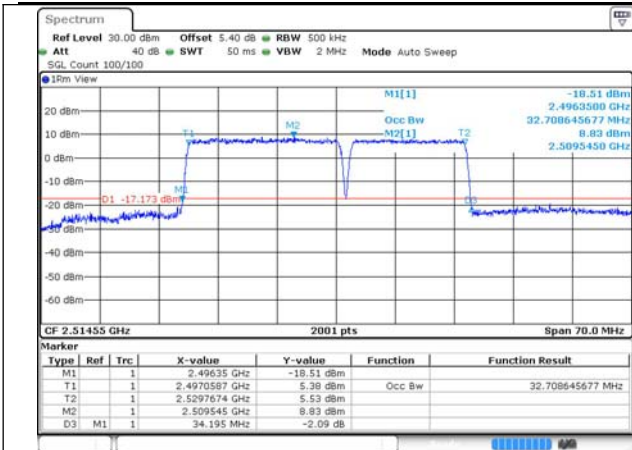
41-41-20MHz-15MHz-QPSK-QPSK-39750-39921-100 RB#0-75RB#0
