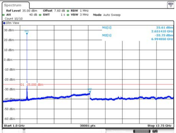
41-41-20MHz-20MHz-QPSK-QPSK-41292-41490 -1RB#0-ORB#0-1000~12750MHz
