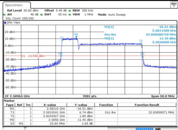
41-41-5MHz-20MHz-64QAM-64QAM-40528-40645-2 5RB#0-100RB#0
