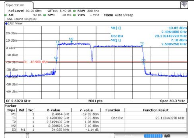
41-41-10MHz-15MHz-256QAM-256QAM-39703-39823-50RB#0-75RB#0
