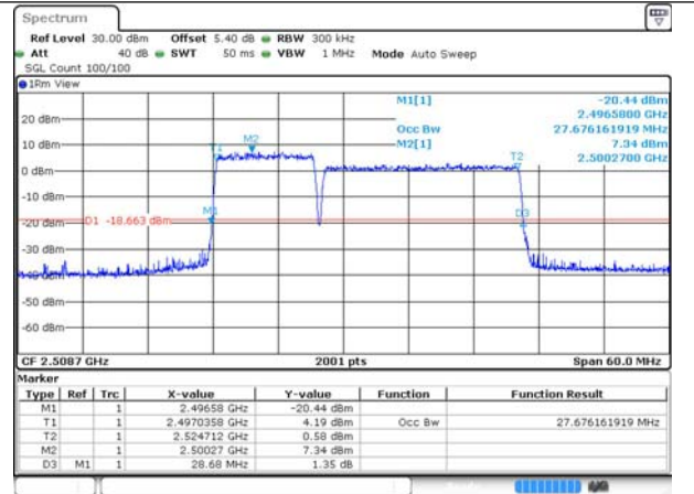
41-41-10MHz-20MHz-256QAM-256QAM-39705-39849-50RB#0-100RB#0
