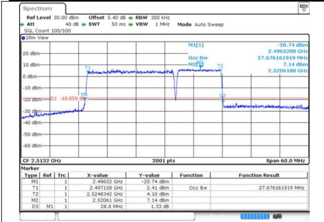
41-41-20MHz-10MHz-64QAM-64QAM-39750-39894-100RB#0-50RB#0
