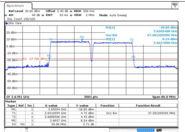
41-41-20MHz-20MHz-16QAM-16QAM-41292-41490-100RB#0-100RB#0
