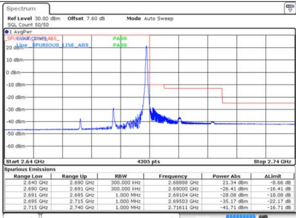
CA_41C_100RB+100RB_QPSK_39750+39948_1R B#0+0RB#0
