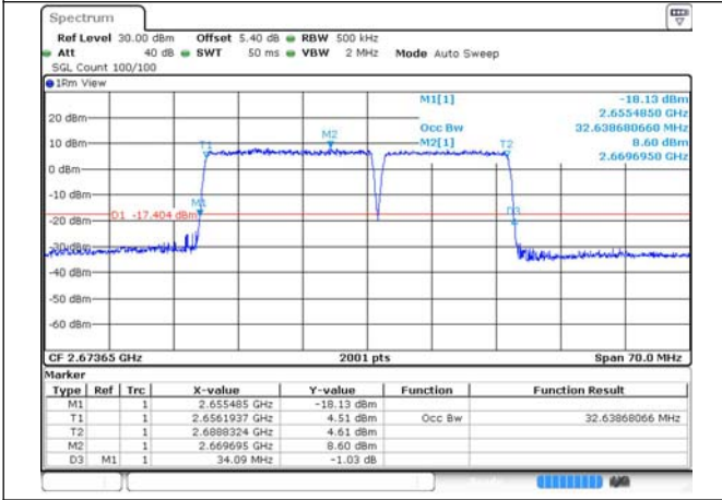
41-41-20MHz-15MHz-64QAM-64QAM-41341-41512-100RB#0-75RB#0
