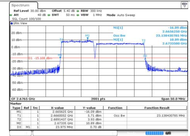
41-41-10MHz-15MHz-16QAM-16QAM-41395-41515-50RB#0-75RB#0
