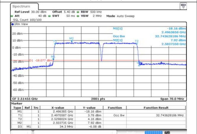
41-41-20MHz-15MHz-16QAM-16QAM-39750-39921-100RB#0-75RB#0
