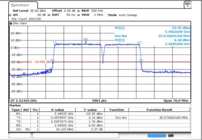
41-41-20MHz-15MHz-256QAM-256QAM-39750-39921-100RB#0-75RB#0
