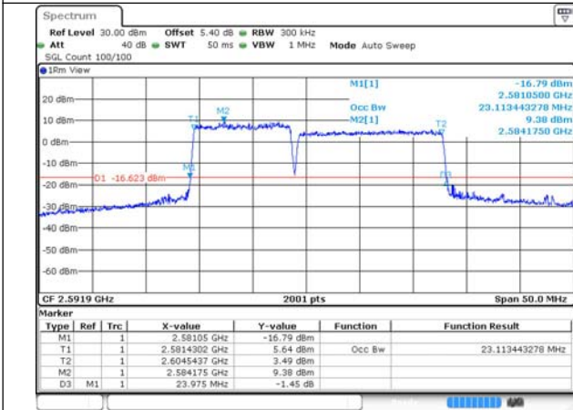
41-41-10MHz-15MHz-16QAM-16QAM-40549-40669-50RB#0-75RB#0
