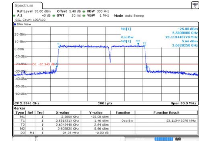
41-41-15MHz-10MHz-256QAM-256QAM-40571-40691-7-75RB#0-50RB#0
