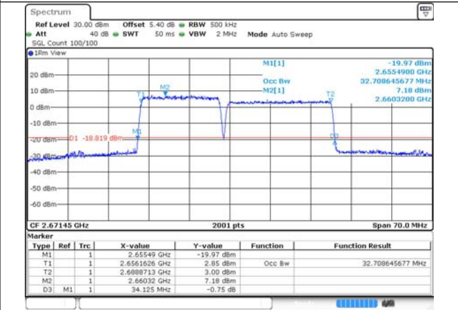
41-41-15MHz-20MHz-256QAM-256QAM-41319-4149-0-75RB#0-100RB#0
