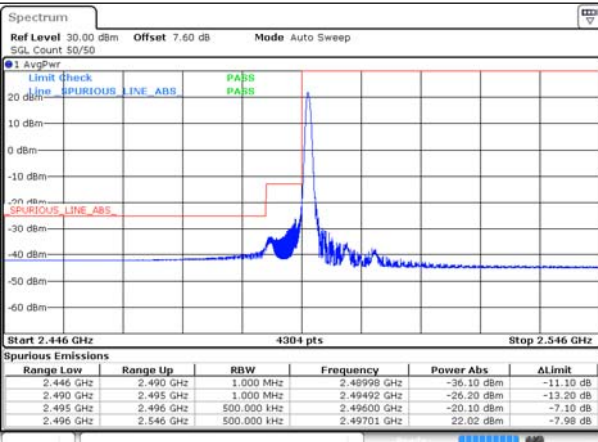
CA_41C_100RB+100RB_QPSK_39750+39948_1R B#0+0RB#0
