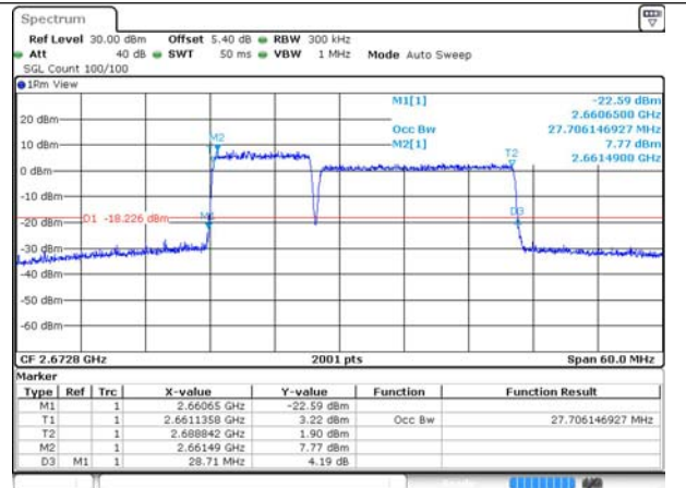
41-41-10MHz-20MHz-256QAM-256QAM-41346-41490-50RB#0-100RB#0
