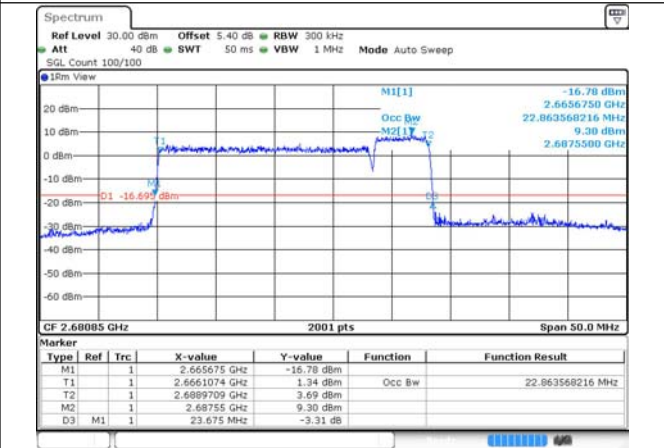
41-41-20MHz-5MHz-256QAM-256QAM-41440-41557-100RB#0-25RB#0
