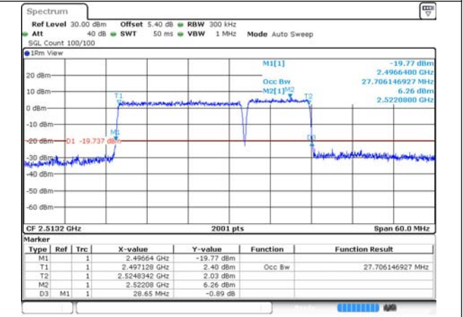
41-41-20MHz-10MHz-256QAM-256QAM-39750-39894-100RB#0-50RB#0
