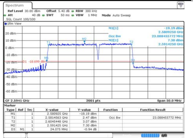
41-41-15MHz-10MHz-64QAM-64QAM-40571-40691-75RB#0-50RB#0
