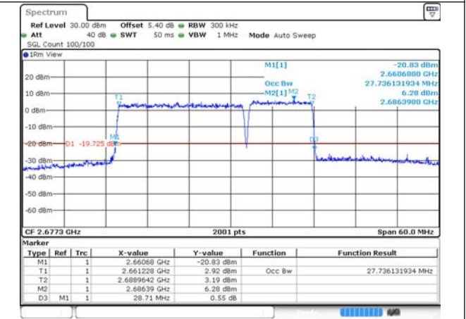
41-41-20MHz-10MHz-256QAM-256QAM-41391-41535-100RB#0-50RB#0
