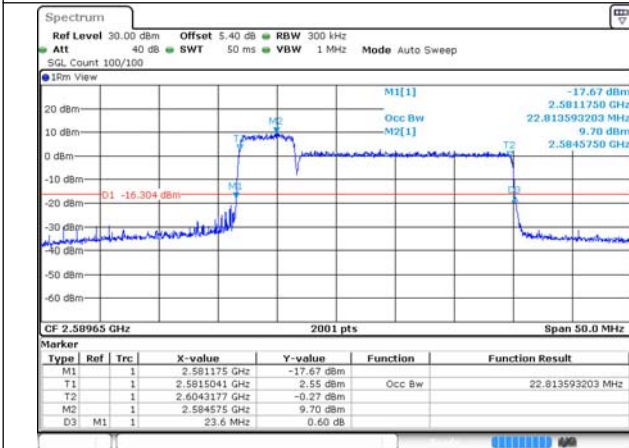
41-41-5MHz-20MHz-256QAM-256QAM-40528-40645 -25RB#0-100RB#0
