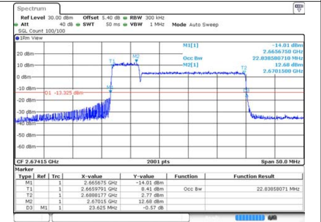
41-41-5MHz-20MHz-16QAM-16QAM-41373-41490-2 5RB#0-100RB#0
