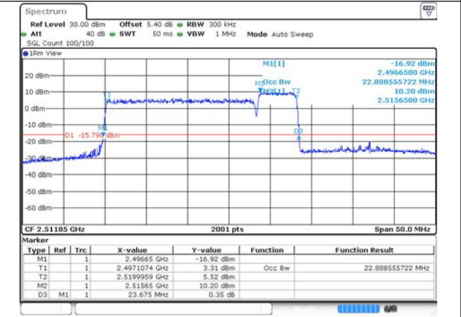
41-41-20MHz-5MHz-16QAM-16QAM-39750-39867-100RB#0-25RB#0
