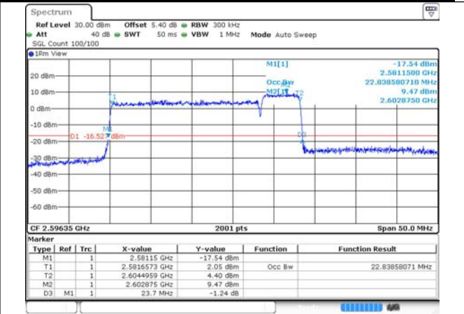
41-41-20MHz-5MHz-64QAM-64QAM-40595-40712-1 00RB#0-25RB#0
