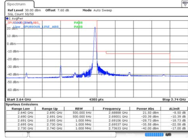
CA_41C_100RB+100RB_QPSK_41292+41490_0R B#0+1RB#99
