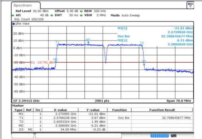
41-41-20MHz-15MHz-256QAM-256QAM-40546-40717-100RB#0-75RB#0
