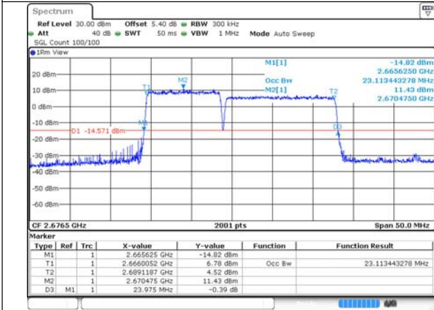
41-41-10MHz-15MHz-QPSK-QPSK-41395-41515-50R B#0-75RB#0
