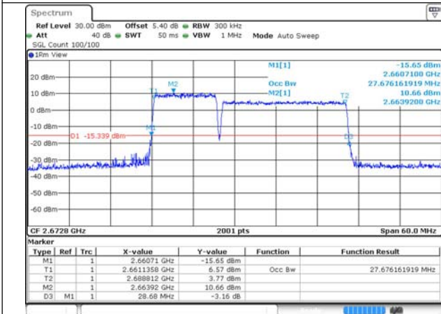
41-41-10MHz-20MHz-QPSK-QPSK-41346-41490-50R B#0-100RB#0
