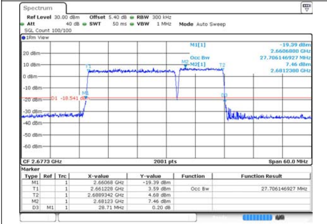
41-41-20MHz-10MHz-64QAM-64QAM-41391-41535-100RB#0-50RB#0
