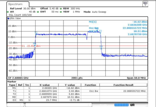
41-41-20MHz-5MHz-16QAM-16QAM-41440-41557-100RB#0-25RB#0
