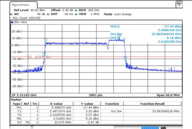
41-41-20MHz-5MHz-256QAM-256QAM-39750-39867-100RB#0-25RB#0
