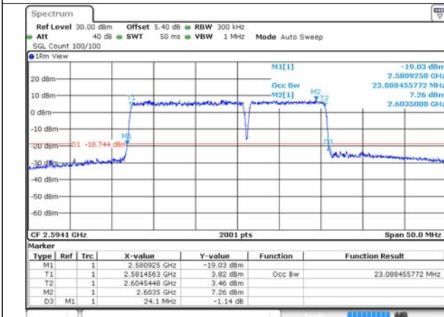
41-41-15MHz-10MHz-16QAM-16QAM-40571-40691-75RB#0-50RB#0
