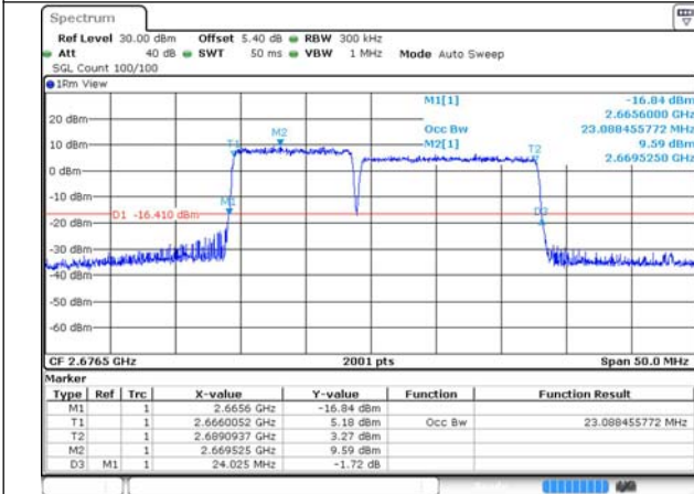
41-41-10MHz-15MHz-64QAM-64QAM-41395-41515-50RB#0-75RB#0
