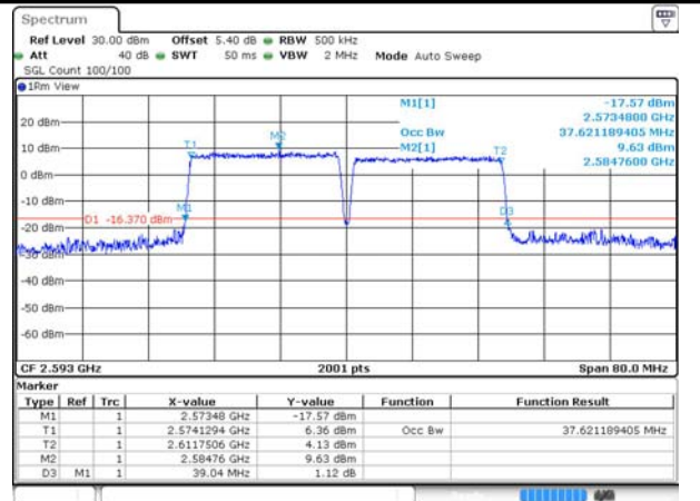
41-41-20MHz-20MHz-QPSK-QPSK-40521-40719-100 RB#0-100RB#0
