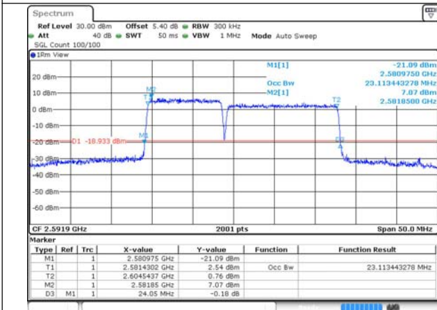
41-41-10MHz-15MHz-256QAM-256QAM-40549-40669-50RB#0-75RB#0
