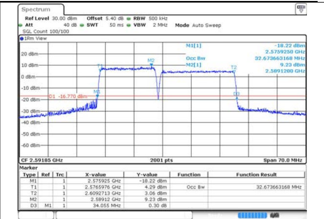
41-41-15MHz-20MHz-64QAM-64QAM-40523-40694-75RB#0-100RB#0
