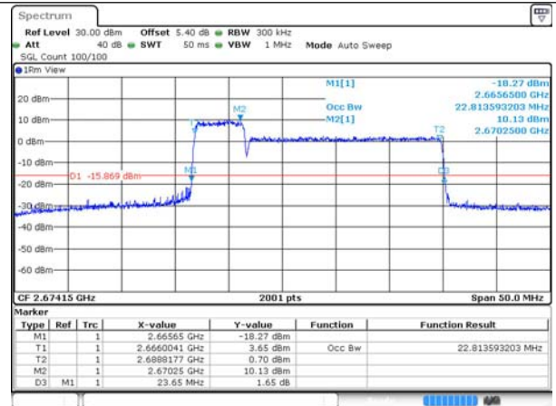
41-41-5MHz-20MHz-256QAM-256QAM-41373-41490 -25RB#0-100RB#0
