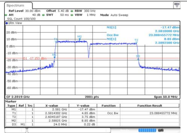
41-41-10MHz-15MHz-64QAM-64QAM-40549-40669-50RB#0-75RB#0
