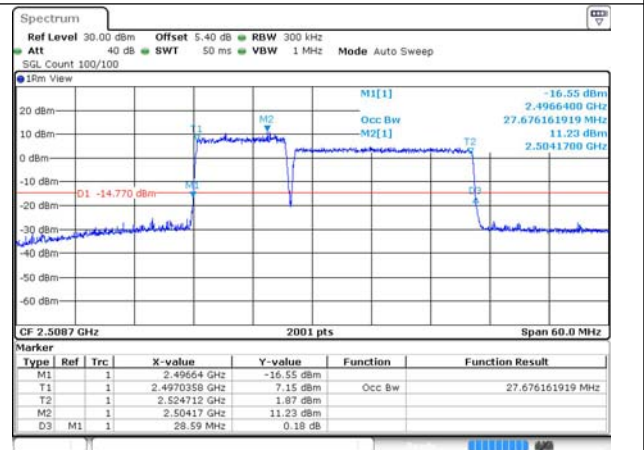
41-41-10MHz-20MHz-16QAM-16QAM-39705-39849-50RB#0-100RB#0
