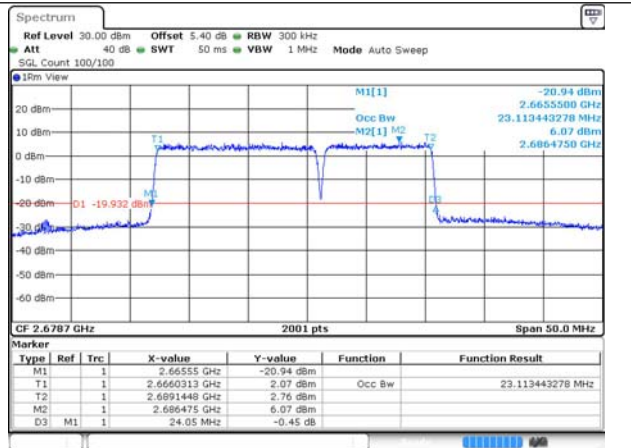
41-41-15MHz-10MHz-256QAM-256QAM-41417-41537-7-75RB#0-50RB#0
