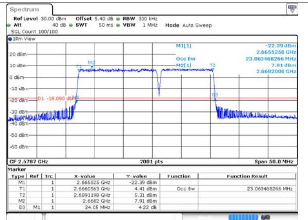
41-41-15MHz-10MHz-16QAM-16QAM-41417-41537-75RB#0-50RB#0
