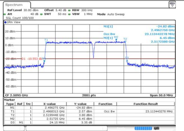
41-41-15MHz-10MHz-256QAM-256QAM-39725-39845-5-75RB#0-50RB#0
