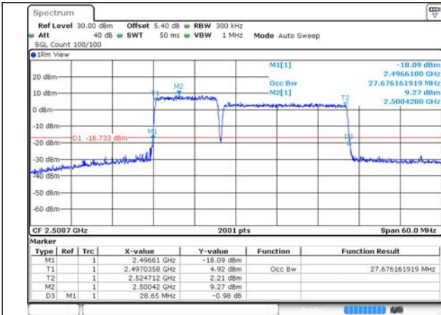
41-41-10MHz-20MHz-64QAM-64QAM-39705-39849-50RB#0-100RB#0
