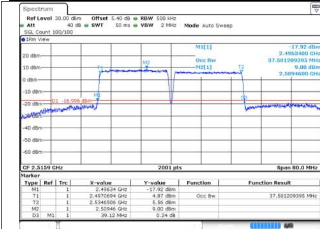
41-41-20MHz-20MHz-QPSK-QPSK-39750-39948-100 RB#0-100RB#0
