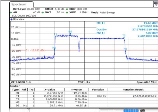
41-41-10MHz-20MHz-256QAM-256QAM-40526-40670-50RB#0-100RB#0
