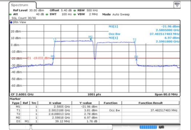
38-38-20MHz-20MHz-16QAM-16QAM-37952-38150-100RB#0-100RB#0
