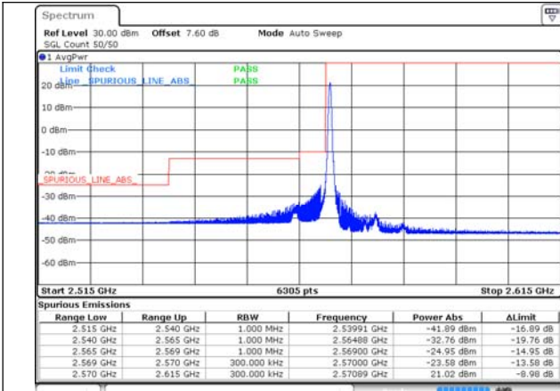
CA_38C_75RB+75RB_QPSK_37825+37975_1RB#0+0RB#0
