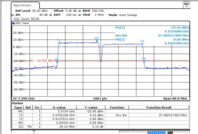
38-38-20MHz-20MHz-16QAM-16QAM-37901-38099-100RB#0-100RB#0
