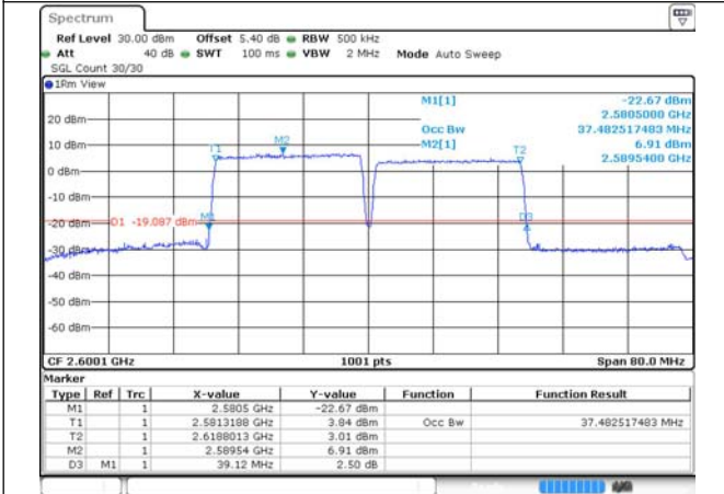
38-38-20MHz-20MHz-64QAM-64QAM-37952-38150-100RB#0-100RB#0
