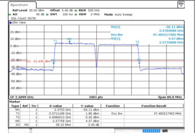
38-38-20MHz-20MHz-256QAM-256QAM-37850-3804-8-100RB#0-100RB#0
