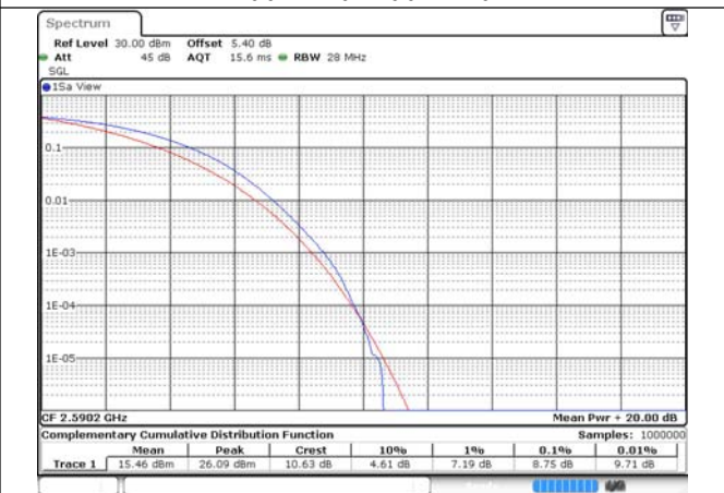
CA_38C_100RB+100RB_256QAM_37952+38150_100RB#0+100RB#0
