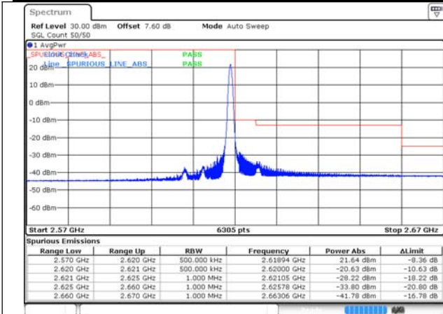
CA_38C_100RB+100RB_QPSK_37952+38150_0R B#0+1RB#99
