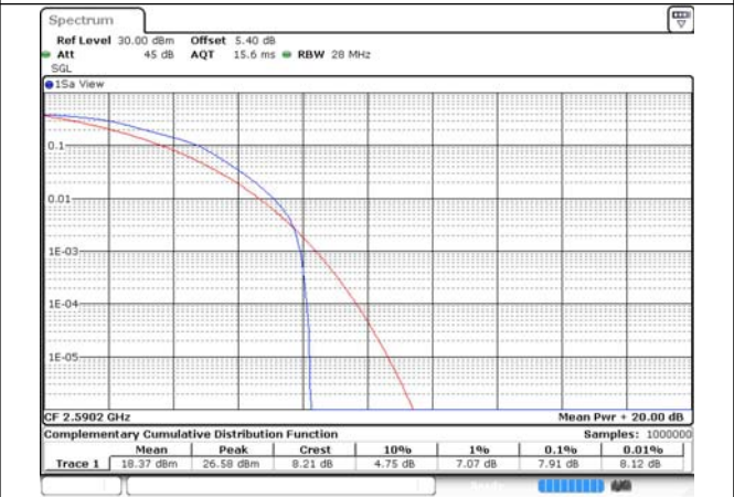
CA_38C_100RB+100RB_16QAM_37952+38150_100RB#0+100RB#0
