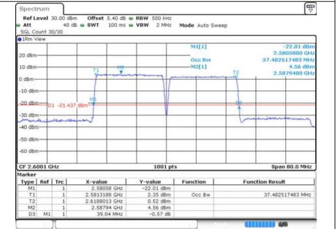
38-38-20MHz-20MHz-256QAM-256QAM-37952-3815-0-100RB#0-100RB#0
