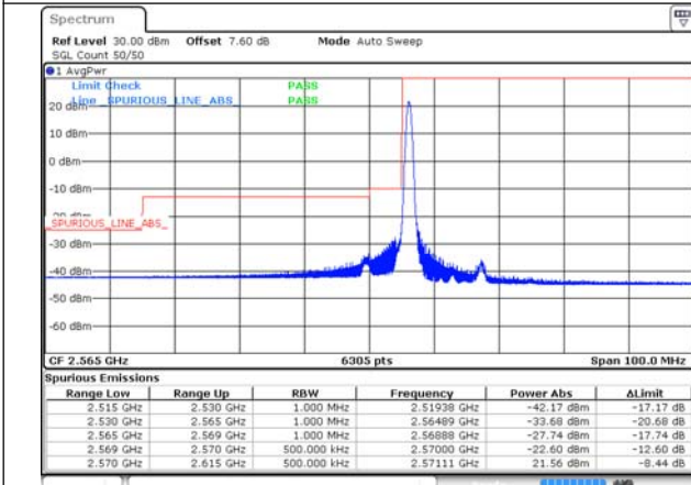
CA_38C_100RB+100RB_QPSK_37850+38048_1RB#0+0RB#0
