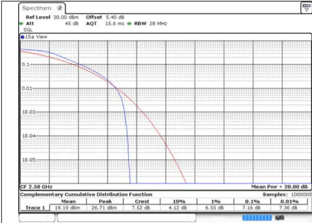
CA_38C_100RB+100RB_QPSK_37850+38048_100RB#0+100RB#0
