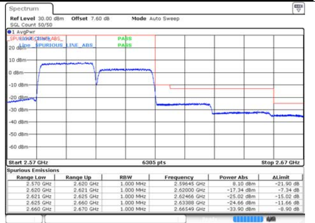
CA_38C_100RB+100RB_QPSK_37952+38150_100 RB#0+100RB#0
