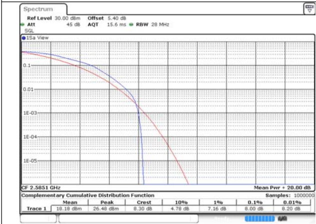
CA_38C_100RB+100RB_16QAM_37901+38099_100RB#0+100RB#0
