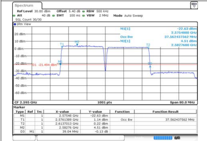
38-38-20MHz-20MHz-256QAM-256QAM-37901-3809-9-100RB#0-100RB#0
