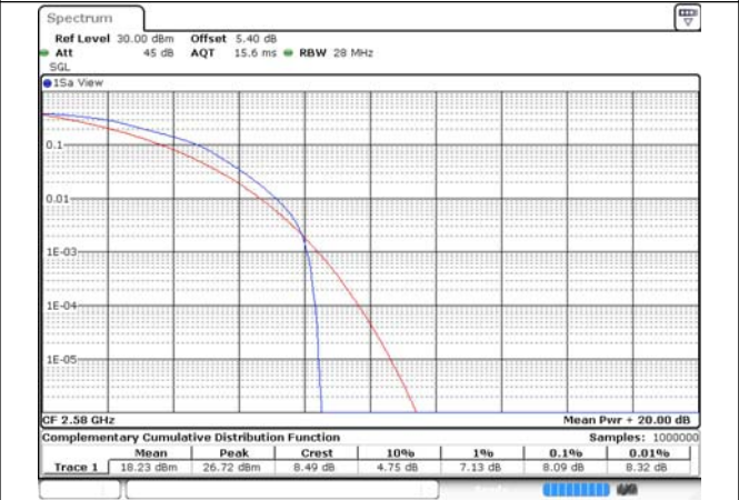
CA_38C_100RB+100RB_16QAM_37850+38048_100RB#0+100RB#0
