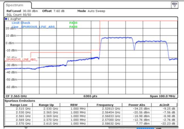
CA_38C_100RB+100RB_QPSK_37850+38048_100RB#0+100RB#0
