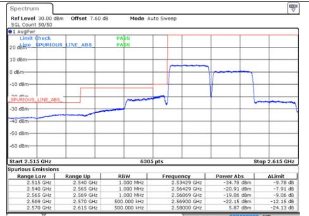
CA_38C_75RB+75RB_QPSK_37825+37975_75RB#0+75RB#0
