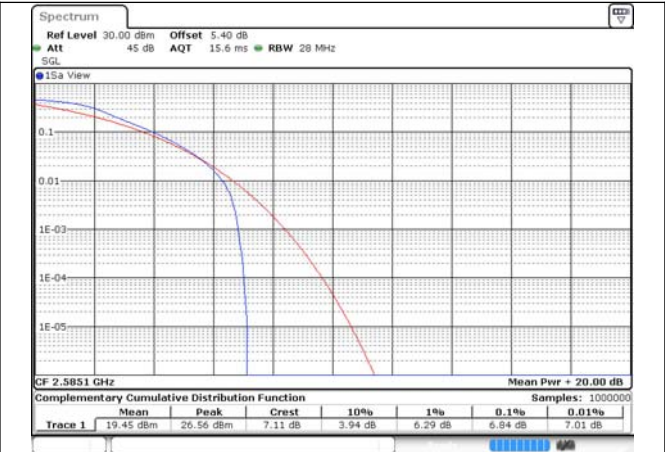
CA_38C_100RB+100RB_QPSK_37901+38099_100RB#0+100RB#0
