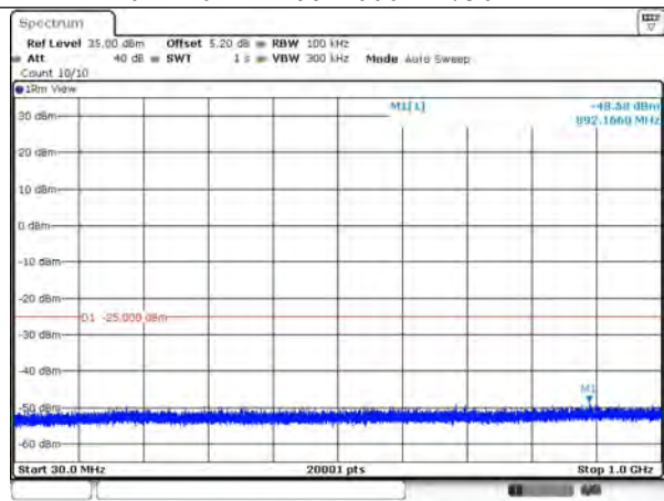
7-7-20MHz-20MHz-QPSK-QPSK-21152-21350 -100RB#0-100RB#0-30~1000MHz
