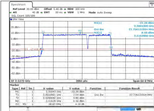
7-7-20MHz-10MHz-QPSK-QPSK-20850-20994-100R B#0-50RB#0
