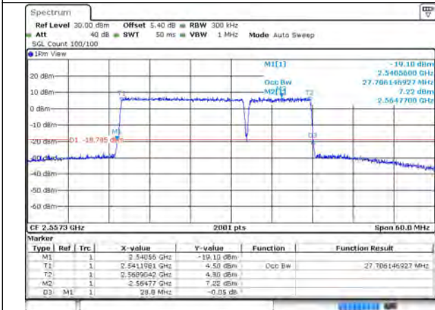
7-7-20MHz-10MHz-64QAM-64QAM-21251-21395-10 ORB#0-50RB#0
