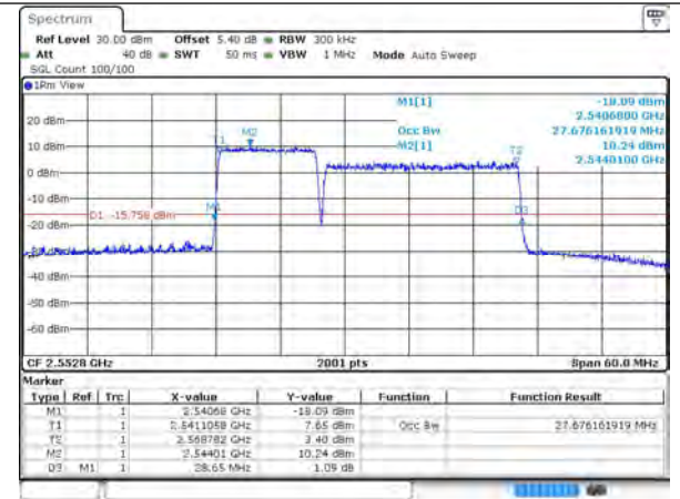
7-7-10MHz-20MHz-16QAM-16QAM-20805-20949-50RB#0-100RB#0
