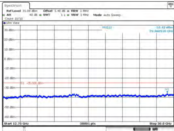
7-7-20MHz-20MHz-QPSK-QPSK-21152-21350 -100RB#0-100RB#0-12750~30000MHz
