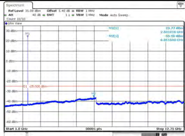
7-7-20MHz-20MHz-QPSK-QPSK-20850-21048 -1RB#0-ORB#0-1000~12750MHz
