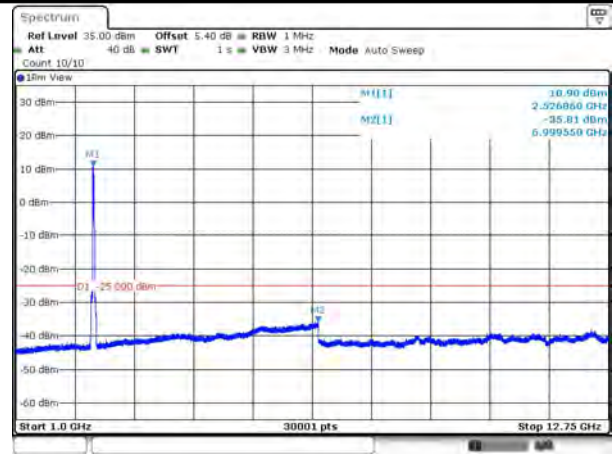
7-7-20MHz-20MHz-QPSK-QPSK-21001-21199 -100RB#0-100RB#0-1000~12750MHz
