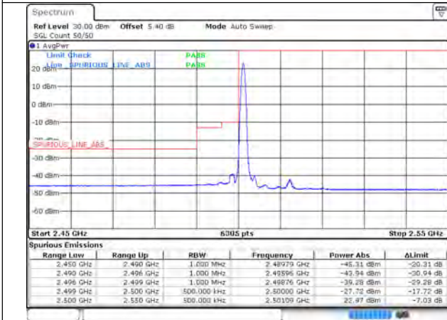
CA_7C_75RB+75RB_QPSK_21225+21375_0RB#0+1RB#74
