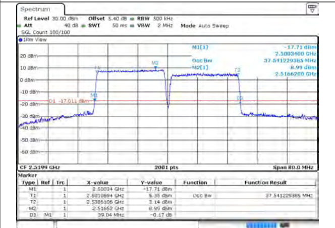
7-7-20MHz-20MHz-16QAM-16QAM-20850-21048-10ORB#0-100RB#0
