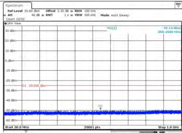
7-7-20MHz-20MHz-QPSK-QPSK-21001-21199 -ORB#0-1RB#99-30~1000MHz
