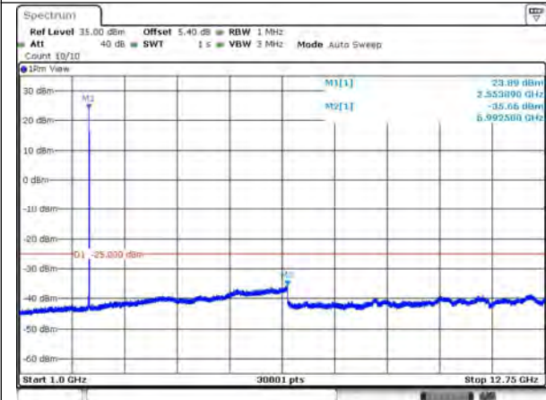
7-7-20MHz-20MHz-QPSK-QPSK-21001-21199 -ORB#0-1RB#99-1000~12750MHz
