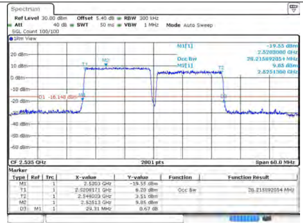
7-7-15MHz-15MHz-QPSK-QPSK-21025-21175-75RB#0-75RB#0
