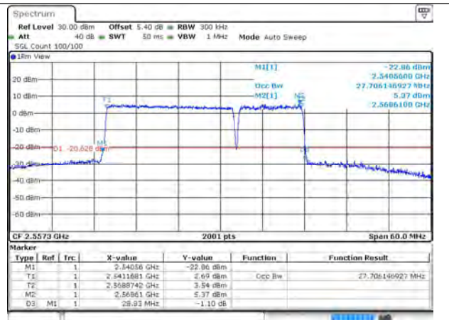
7-7-20MHz-10MHz-256QAM-256QAM-21251-21395-100RB#0-50RB#0
