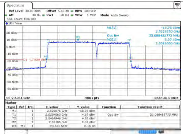
7-7-15MHz-10MHz-64QAM-64QAM-21051-21171-75 RB#0-50RB#0
