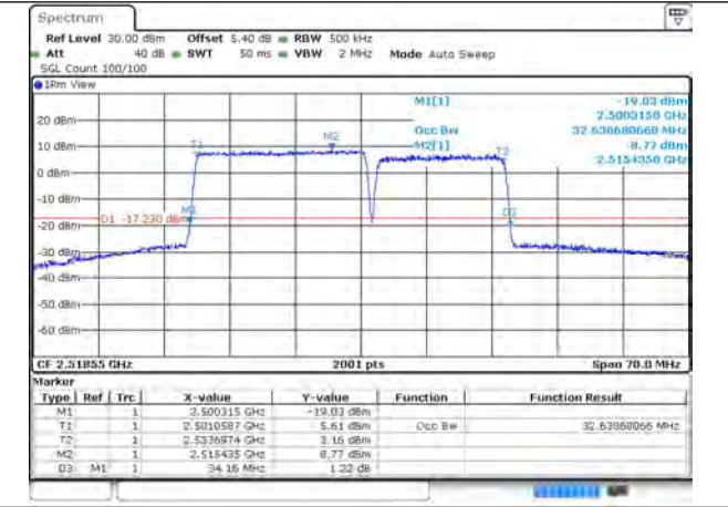
7-7-20MHz-15MHz-16QAM-16QAM-20850-21021-10 ORB#0-75RB#0
