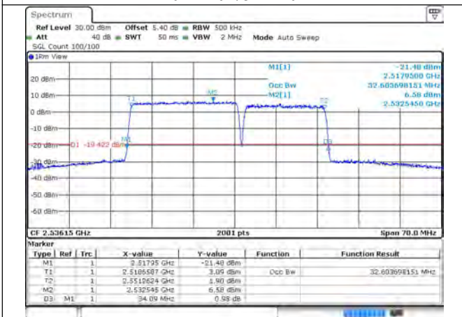
7-7-20MHz-15MHz-256QAM-256QAM-21026-21197-100RB#0-75RB#0
