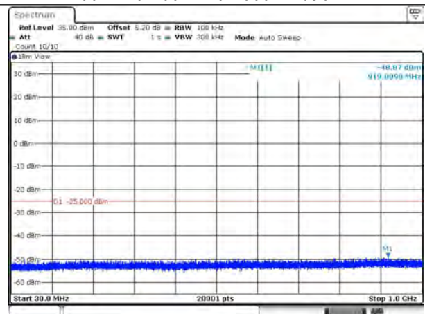
7-7-20MHz-20MHz-QPSK-QPSK-21001-21199 -1RB#0-0RB#0-30~1000MHz
