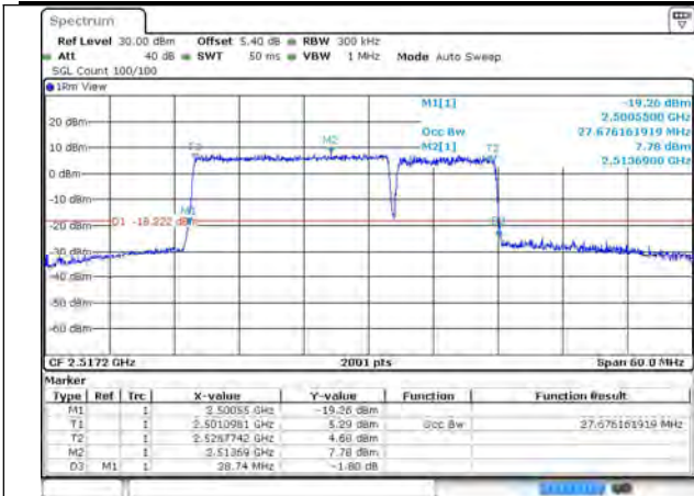
7-7-20MHz-10MHz-64QAM-64QAM-20850-20994-10 ORB#0-50RB#0
