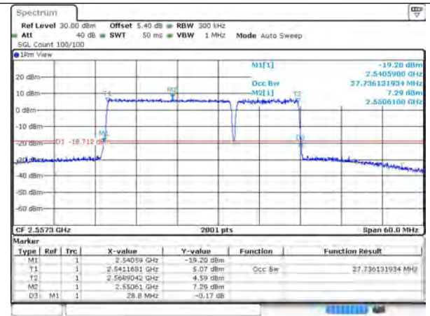
7-7-20MHz-10MHz-16QAM-16QAM-20850-20994-10 ORB#0-50RB#0
