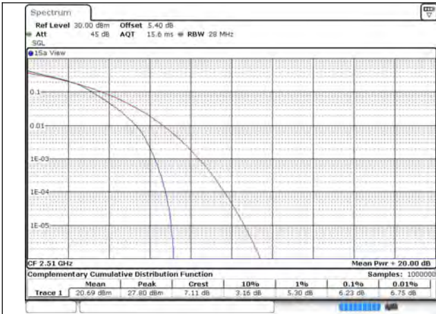
CA_7C_100RB+100RB_64QAM_21048+20850_10ORB#0+100RB#0
