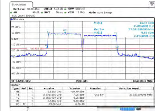
7-7-20MHz-20MHz-QPSK-QPSK-21152-21350-100RB#0-100RB#0
