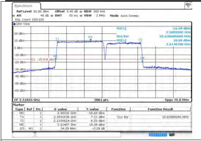
7-7-20MHz-15MHz-QPSK-QPSK-20850-21021-100R B#0-75RB#0
