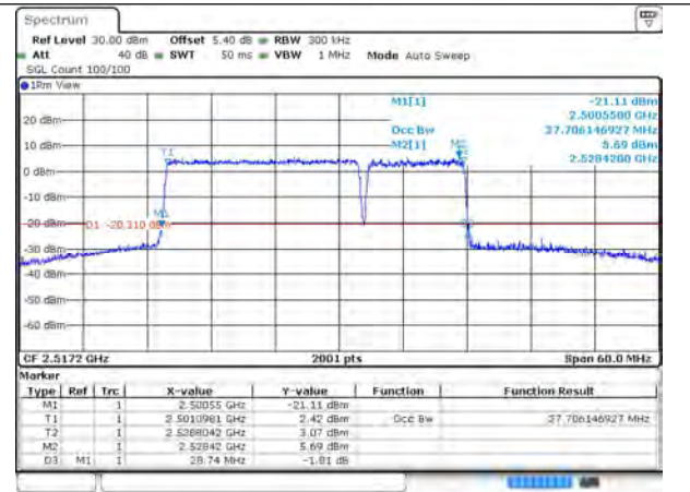
7-7-20MHz-10MHz-256QAM-256QAM-20850-20994-100RB#0-50RB#0
