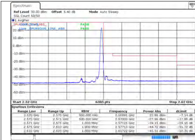
CA_7C_100RB+100RB_QPSK_21152+21350_0RB #0+1RB#99
