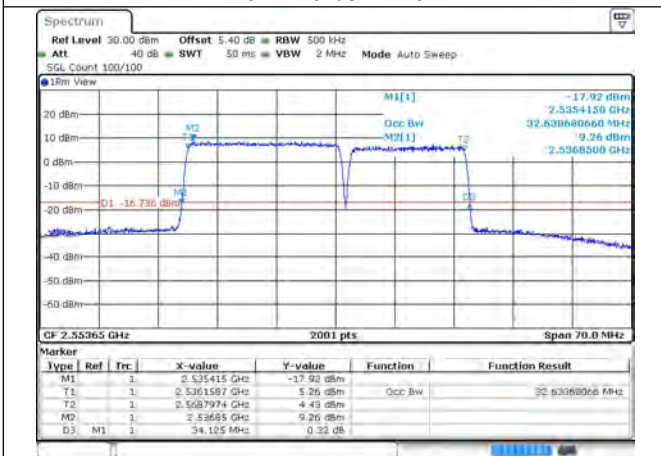
7-7-20MHz-15MHz-64QAM-64QAM-21201-21372-10 ORB#0-75RB#0
