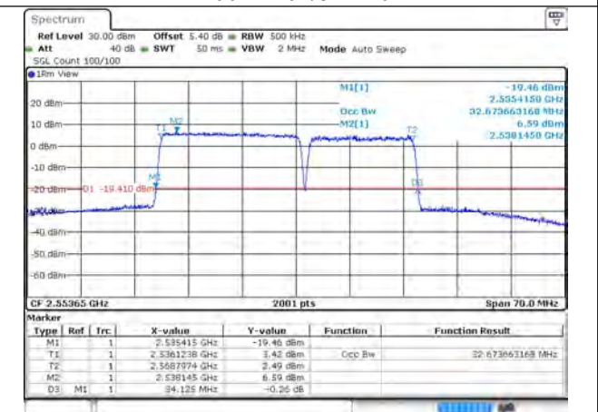
7-7-20MHz-15MHz-256QAM-256QAM-21201-21372-100RB#0-75RB#0
