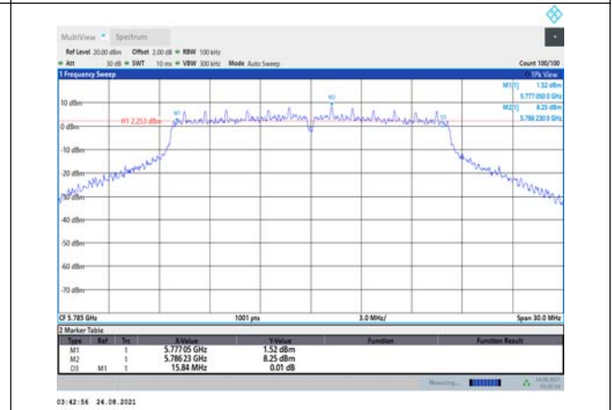
Test Mode:802.11a Ant7
