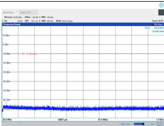
Test Mode:802.11b Ant7 CH11
