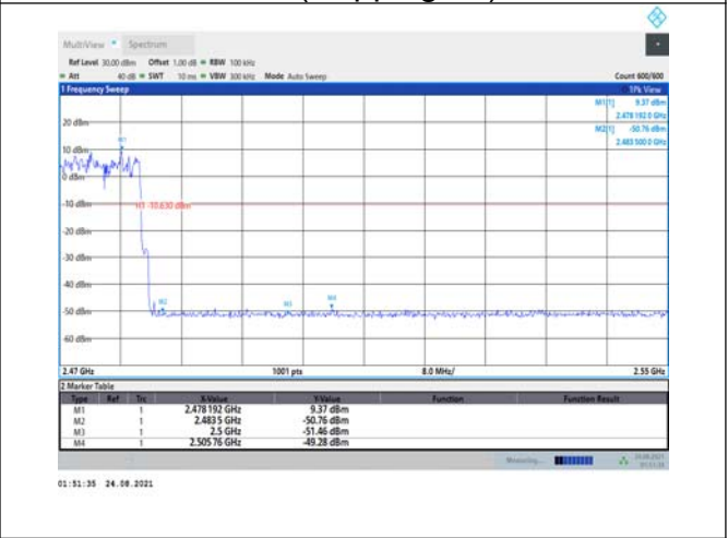
CH78(Hopping on)
