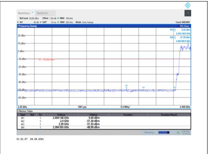
CH0(Hopping on)
