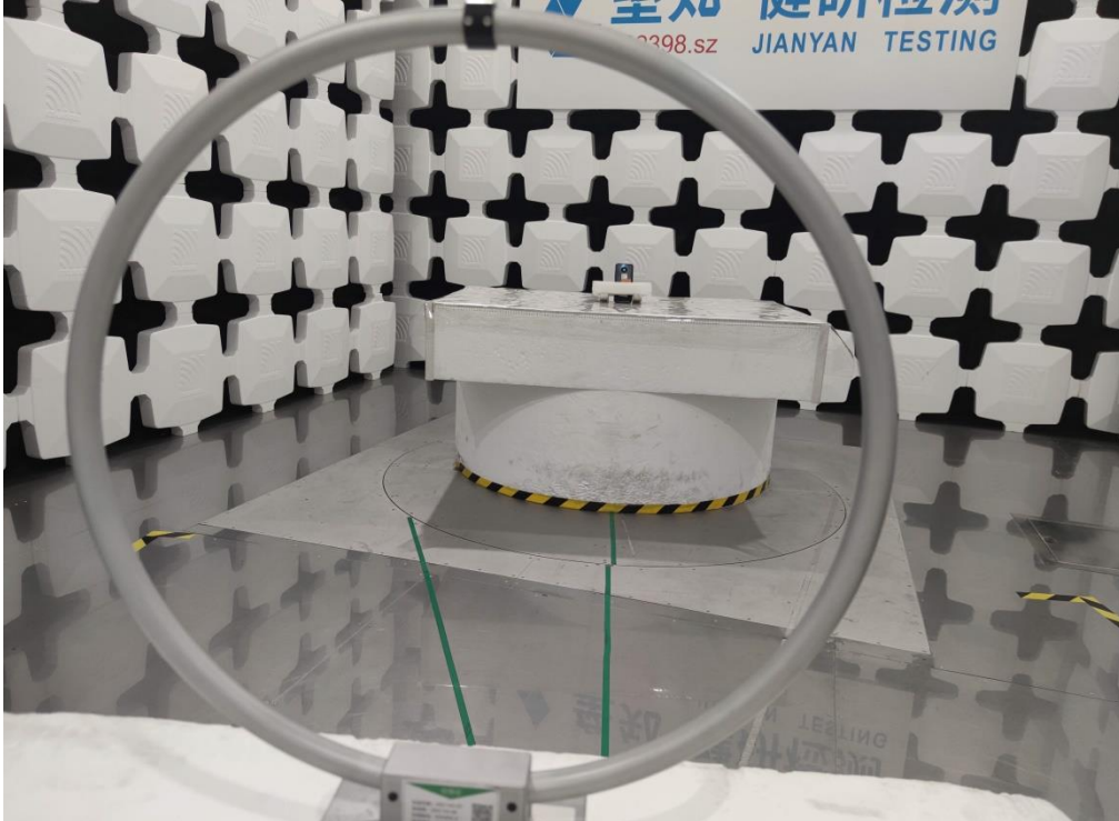
Radiated Emission 9KHz~30MHz
