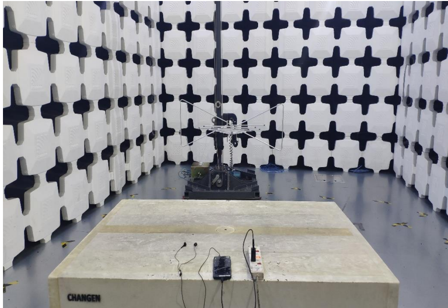
3. Radiated Emissions (Part 15B, Camera/Video Player /GSM receiver/WCDMA receiver/LTE receiver,30MHz-1GHz)
