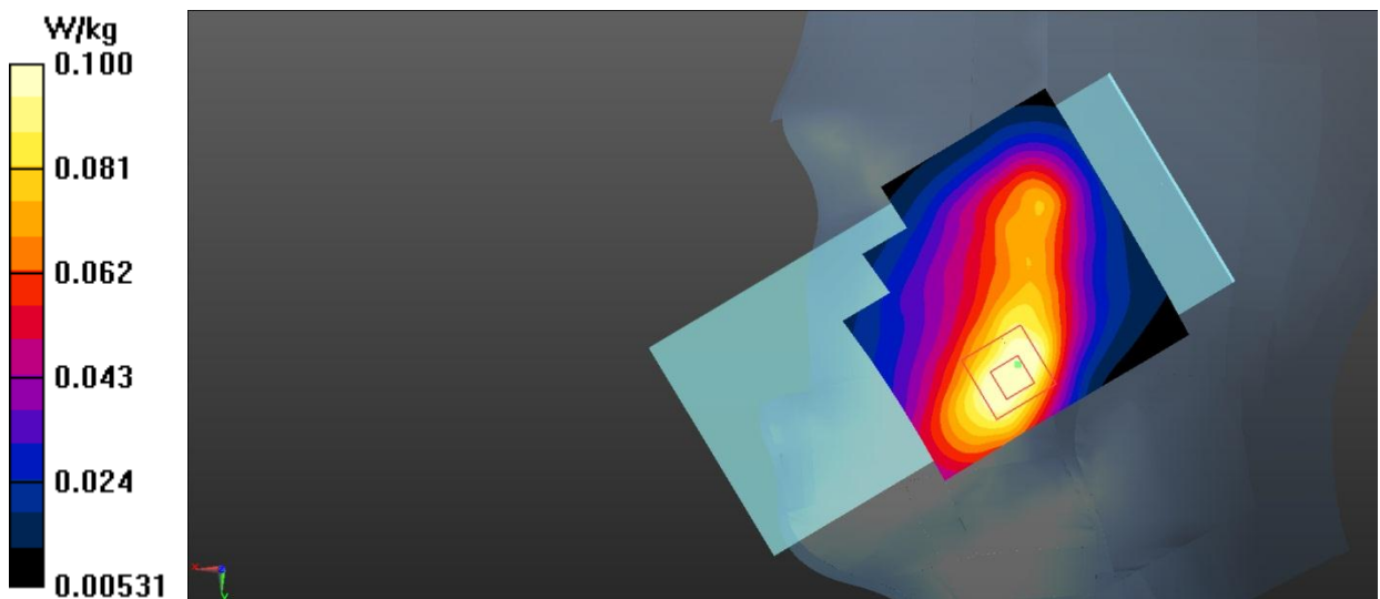
Fig.3 GSM 1900 Head
