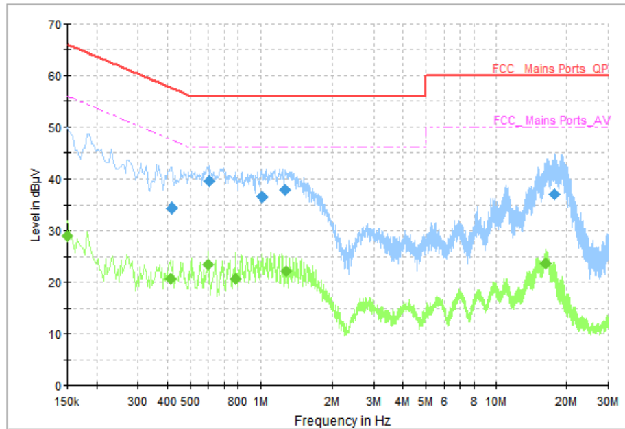
Fig. 86 AC Powerline Conducted Emission (Traffic, AE3, 120V)
