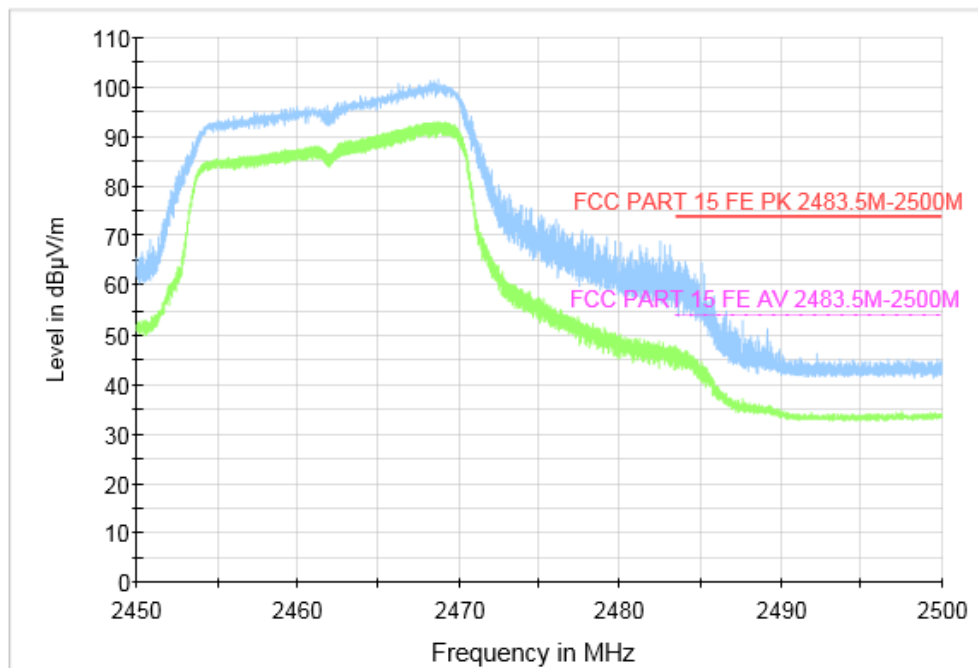
Fig.49 Radiated Restricted Band (802.11g, CH11, 2.45GHz~2.5GHz)
