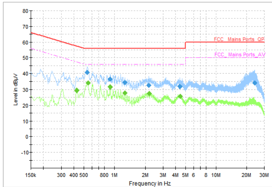
Fig.62 AC Power line Conducted Emission (Idle), LE 1M, A2-1, A3-1
