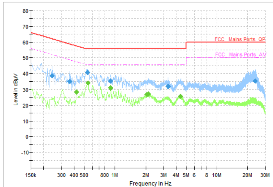
Fig.61 AC Power line Conducted Emission (Traffic), LE 1M, A2-1, A3-1
