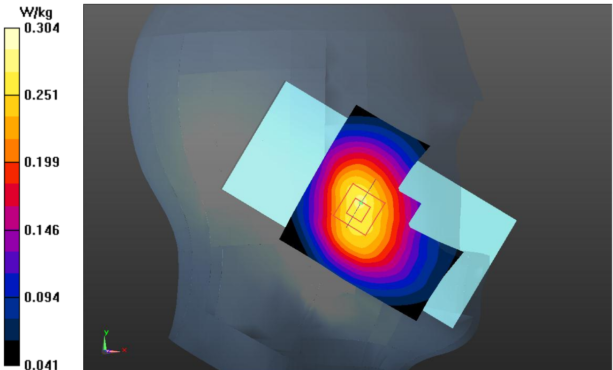
Fig.1 GSM 850 Head
