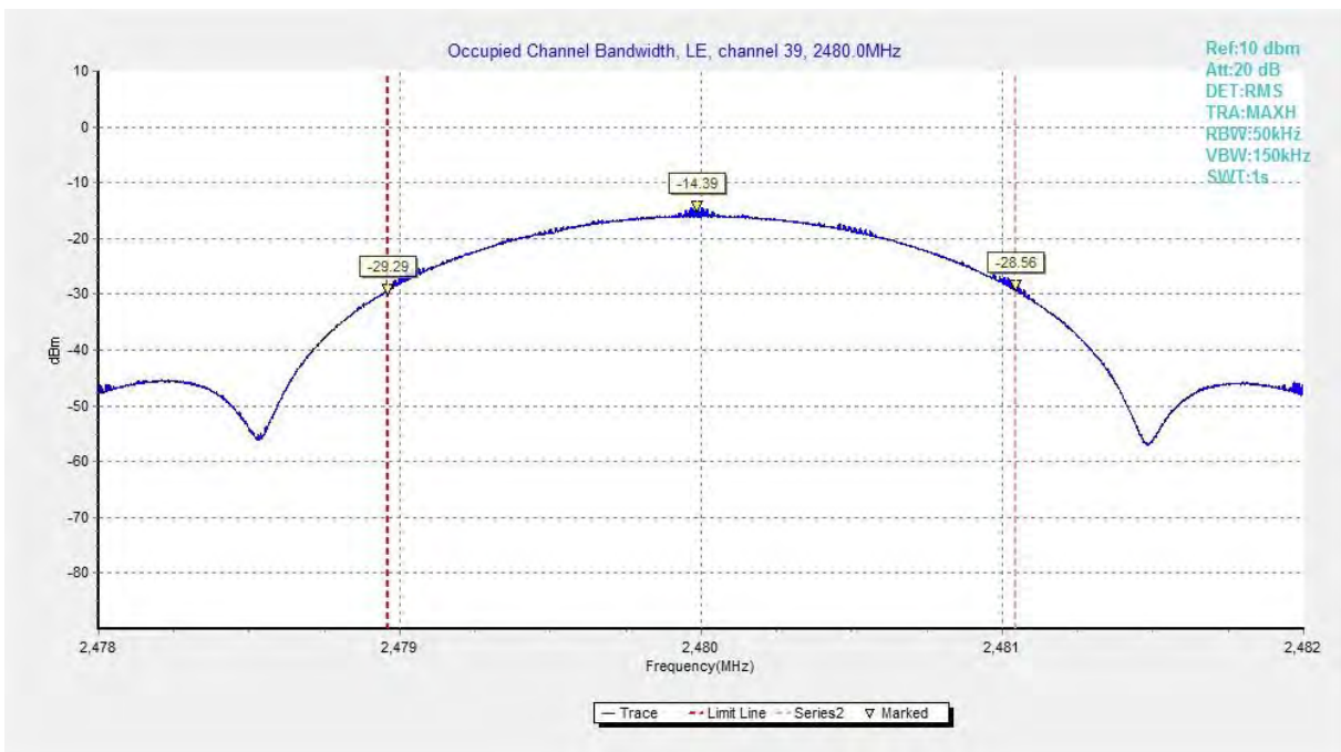
Fig.74 99% Occupied Bandwidth: GFSK, Channel 39, LE 2M
