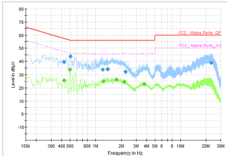
Fig.68 AC Power line Conducted Emission (Idle), LE 2M, A2-2, A3-2
