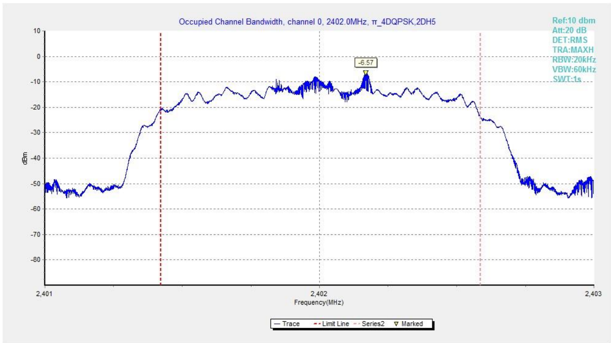
Fig. 100 99% Occupied Bandwidth ( \pi/4 DQPSK, Ch 0)
