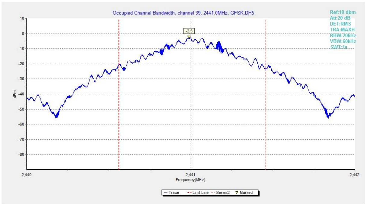
Fig. 98 99% Occupied Bandwidth (GFSK, Ch 39)
