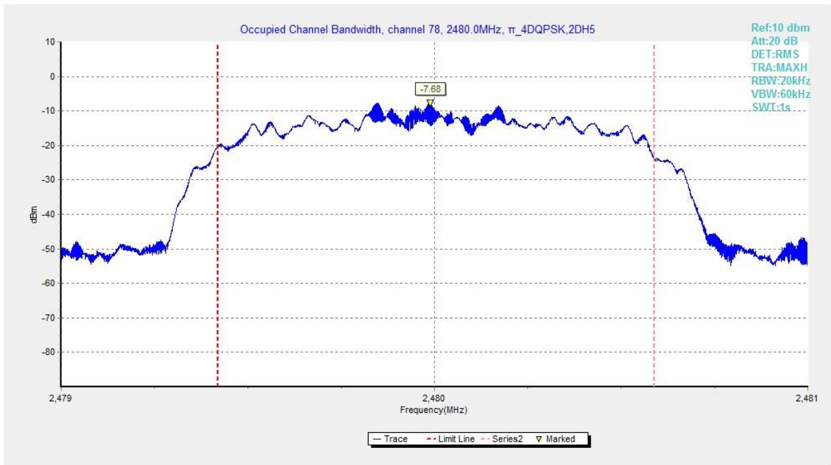
Fig. 102 99% Occupied Bandwidth ( \pi/4 DQPSK, Ch 78)
