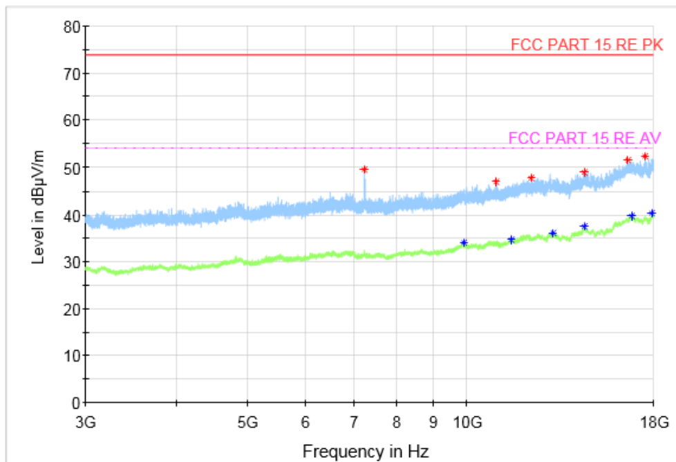
Fig.51 Radiated Spurious Emission (802.11n-HT20, CH1, 3 GHz-18 GHz)
