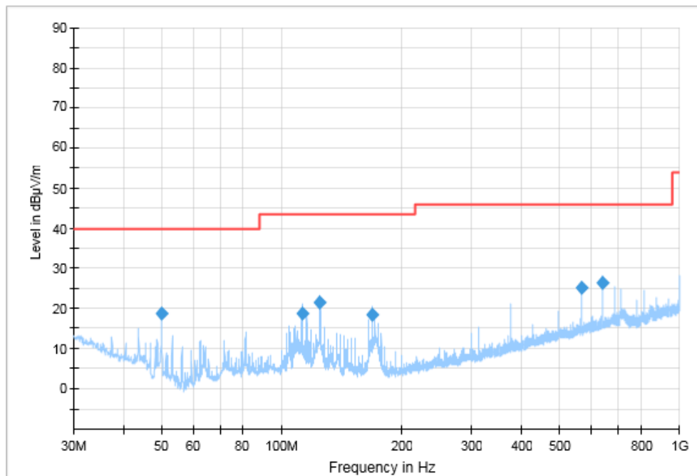
Fig.59 Radiated Spurious Emission (All Channels, 30MHz-1 GHz)
