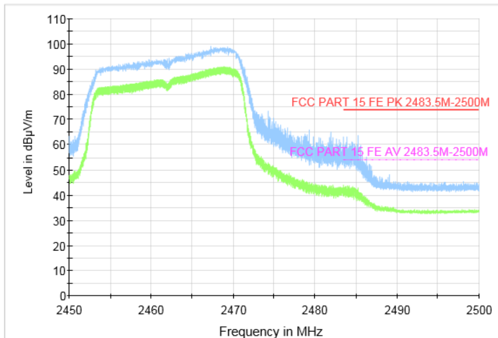
Fig.57 Radiated Restricted Band (802.11n-HT20, CH11, 2.45GHz~2.5GHz)
