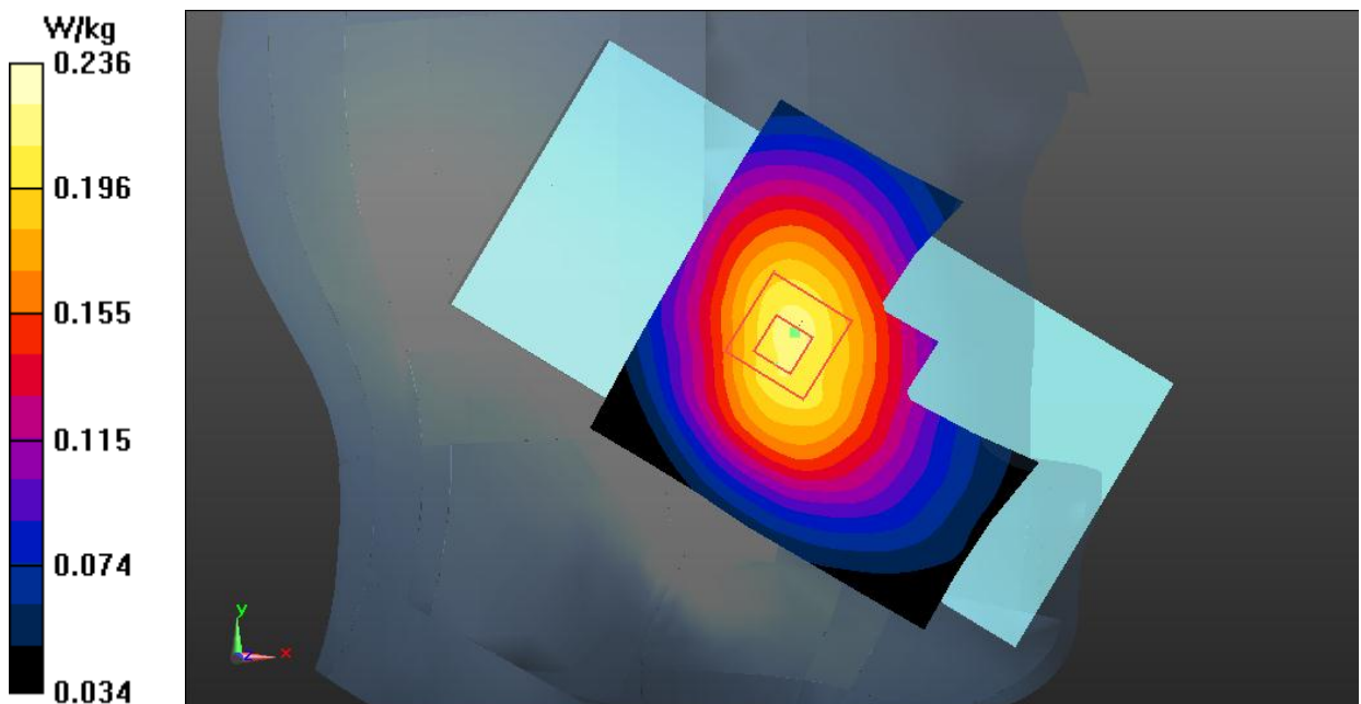
Fig.1 GSM 850 Head
