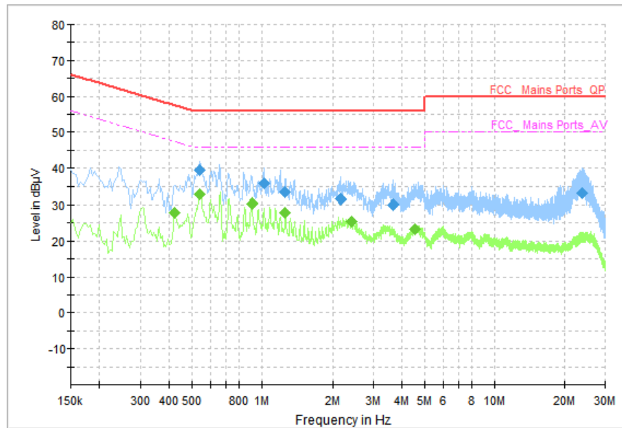
Figure A-6 Conducted Emission (Idle), LE 1M, A2-1, A3-1
