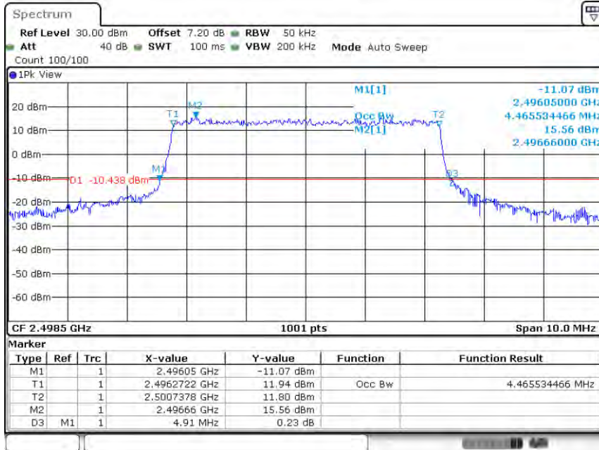
Band41-5MHz-QPSK-39675-25RB#0-4.466
