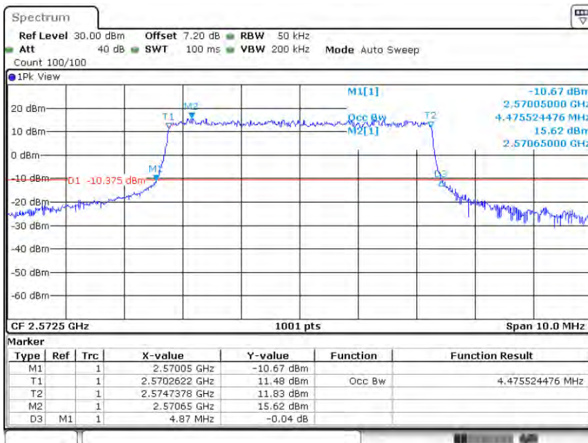
Band38-5MHz-QPSK-37775-25RB#0-4.476
