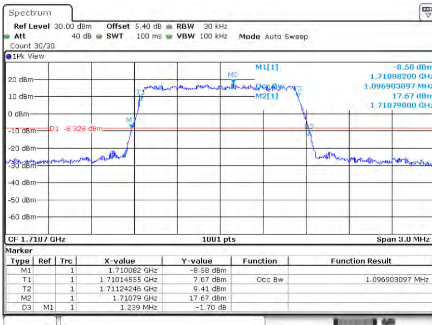
Band4-1.4MHz-QPSK-19957-6RB#0-1.097
