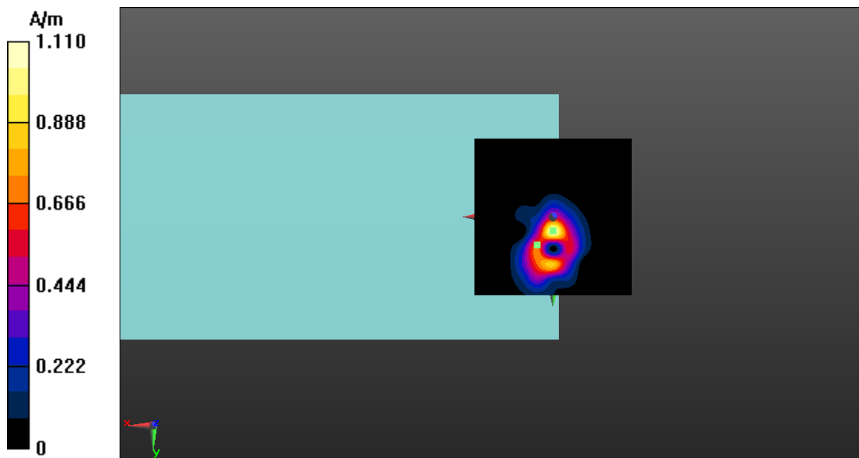
Fig A.14 T-Coil WLAN 2.4G-Z
