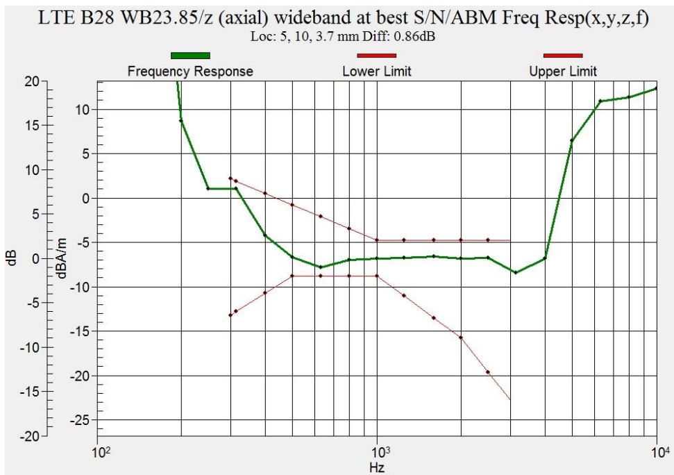
Figure B.12 Frequency Response of LTE Band 28
