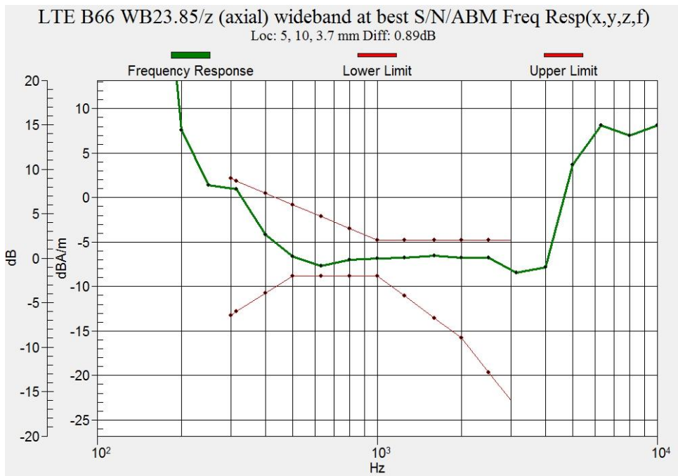
Figure B.13 Frequency Response of LTE Band 66
