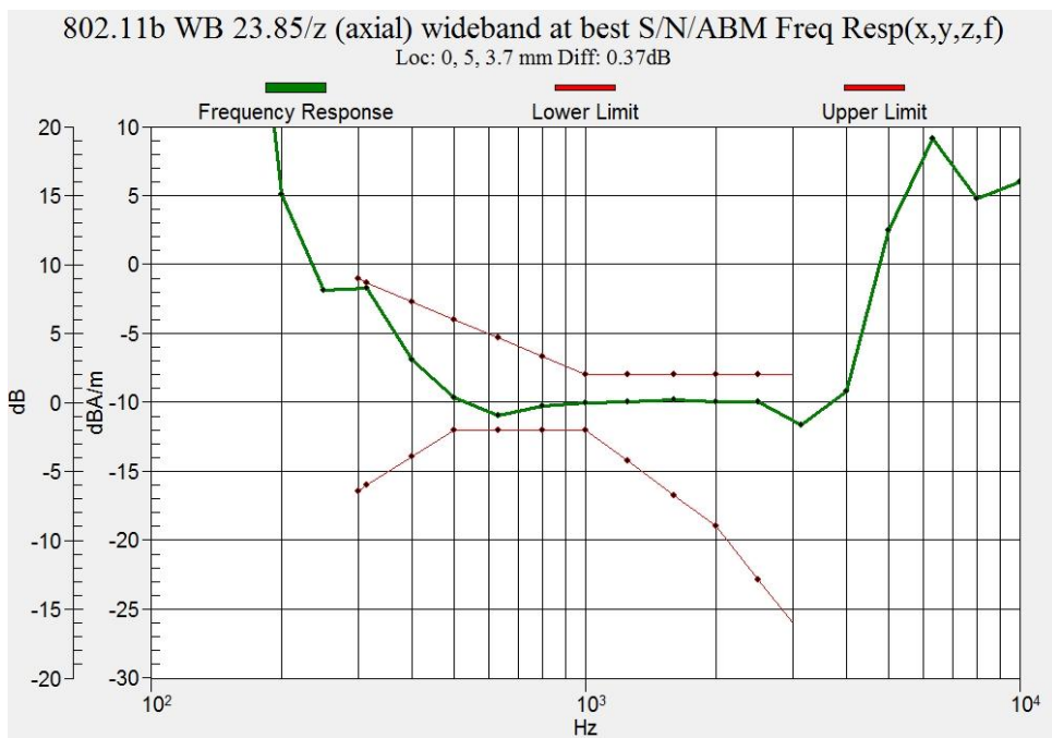
Figure B.14 Frequency Response of WLAN 2.4G
