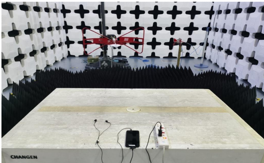
2. Radiated Emissions (Part 15B, Camera,1GHz-18GHz)
