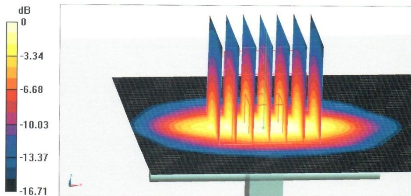
0 dB = 15.9 W/kg = 12.01 dBW/kg
