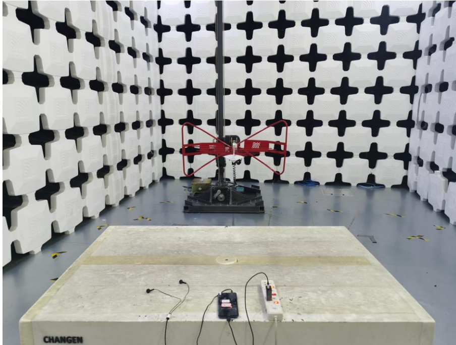
3. Radiated Emissions (Part 15B, Camera/Video Player/GNSS/FM receiver/LTE receiver,30MHz-1GHz)
