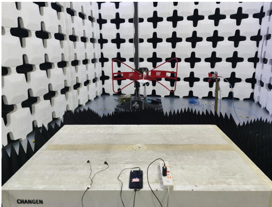
4. Radiated Emissions (Part 15B, Camera/Video Player/GNSS/FM receiver/LTE receiver, 1GHz-18GHz)
