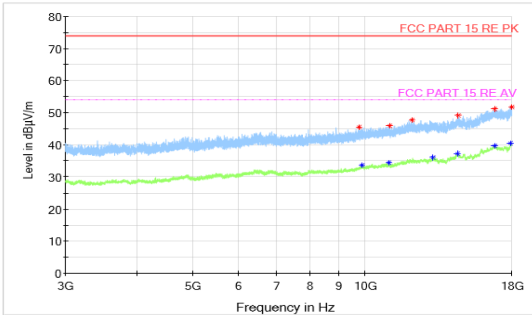
Figure A.1.6. Radiated Emission ( FM receiver , 3GHz to 18GHz)
