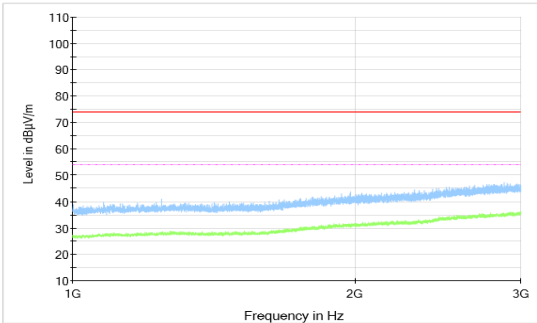
Figure A.1.5. Radiated Emission (FM receiver, 1GHz to 3GHz)
