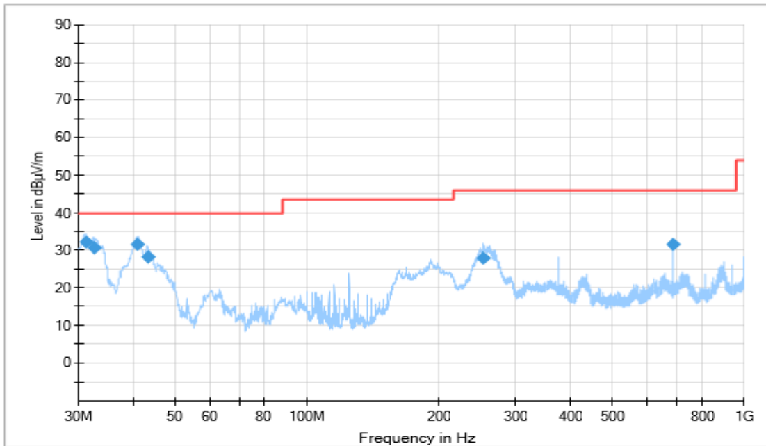
Figure A.1.19. Radiated Emission (Video Player, 30MHz to 1GHz)
