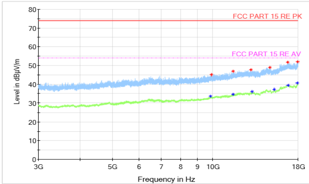
Figure A.1.12. Radiated Emission ( Camera ,3GHz to 18GHz)
