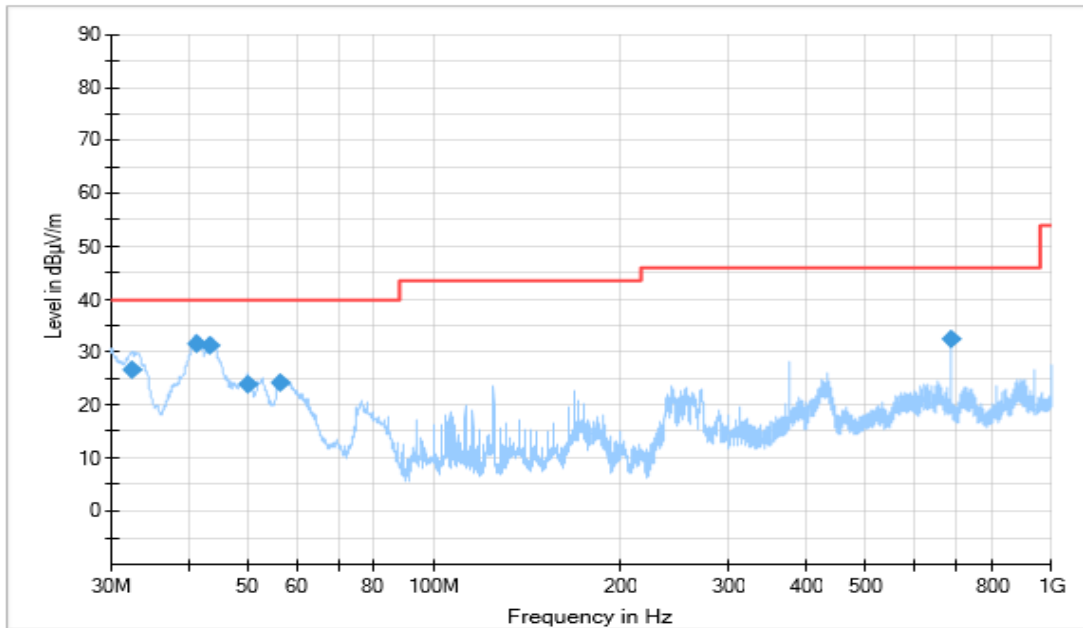
Figure A.1.16. Radiated Emission (GLONASS, 30MHz to 1GHz)
