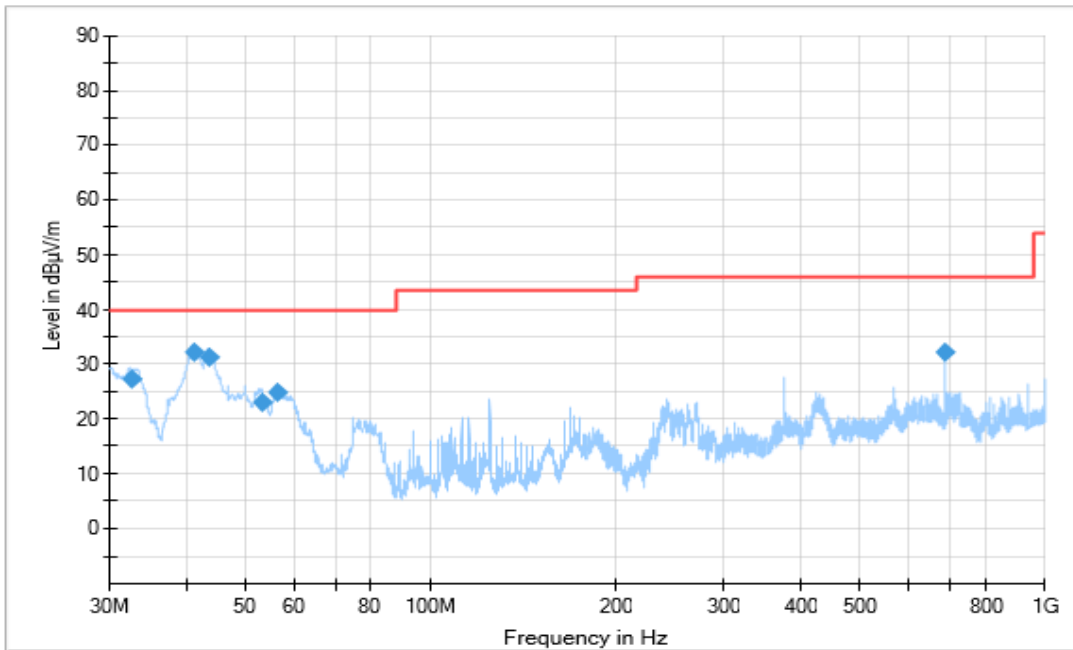
Figure A.1.10. Radiated Emission (Camera , 30MHz to 1GHz)
