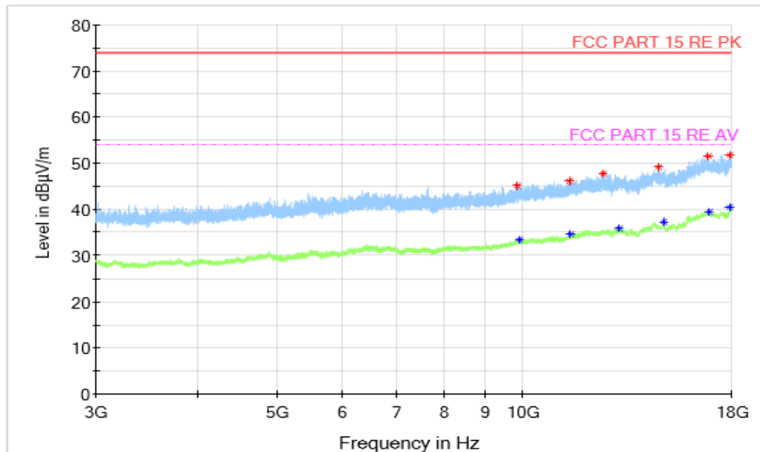
Figure A.1.33. Radiated Emission (Data Transfer : TF Card to PC, 3GHz to 18GHz)
