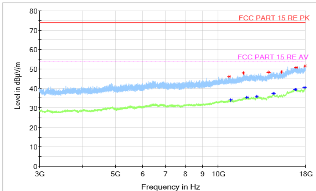
Figure A.1.30. Radiated Emission (Set.8, Data Transfer : PC to TF Card, 3GHz to 18GHz)
