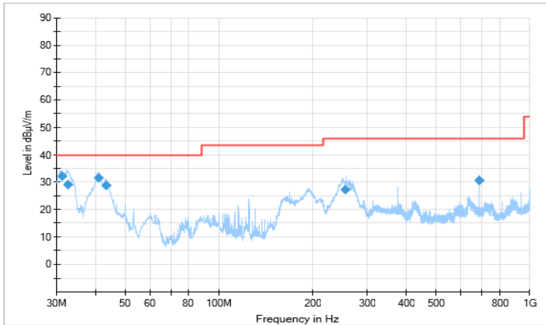
Figure A.1.1. Radiated Emission ( LTE Receiver Band 12, 30MHz to 1GHz)
