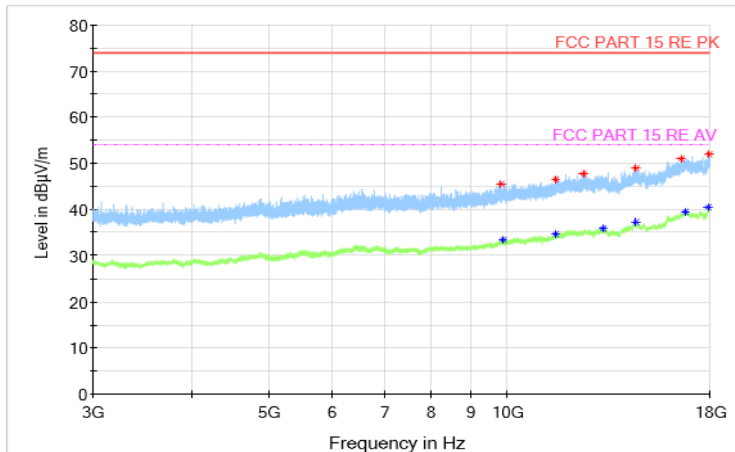
Figure A.1.36. Radiated Emission (Data Transfer : PC to TF Card, 3GHz to 18GHz)
