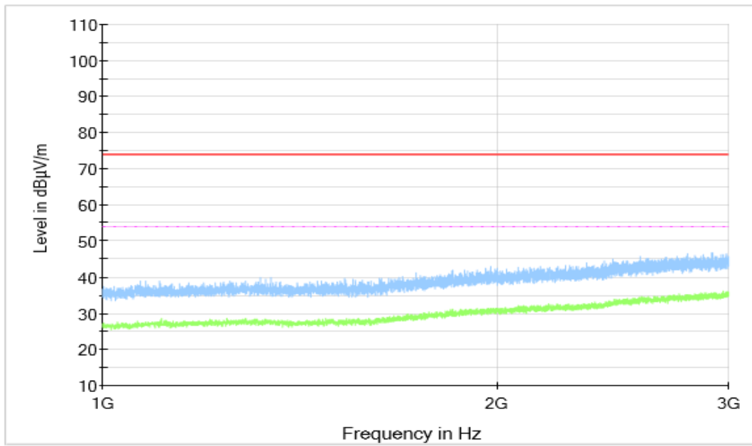
Figure A.1.17. Radiated Emission (GLONASS,1GHz to 3GHz)
