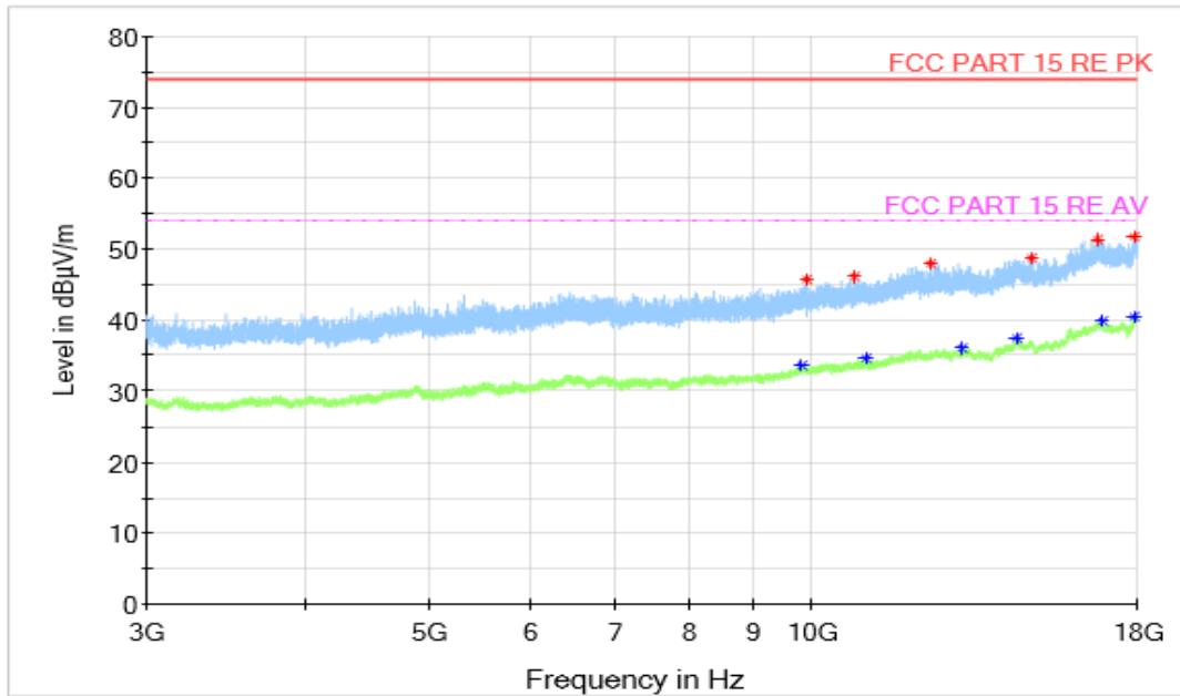
Figure A.1.3. Radiated Emission ( LTE Receiver Band 12, 3GHz to 18GHz)
