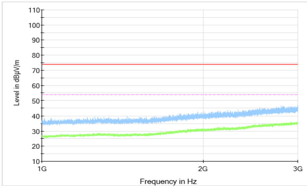
Figure A.1.2. Radiated Emission (LTE Receiver Band 12, 1GHz to 3GHz)
