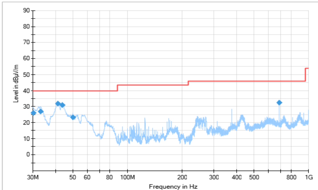
Figure A.1.13. Radiated Emission (GPS, 30MHz to 1GHz)
