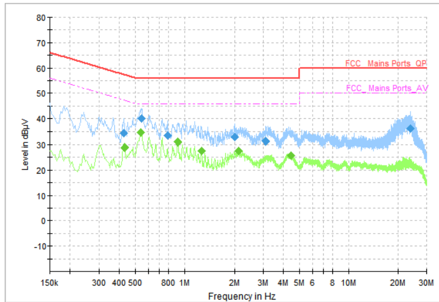
Fig.63 AC Power line Conducted Emission (Traffic), LE 2M, A2-1, A3-1
