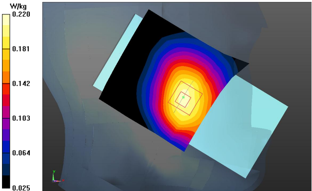
Fig.1 GSM 850 Head
