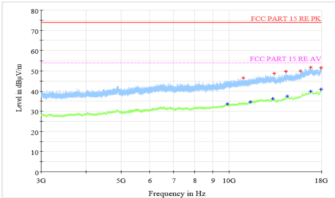
Figure A.1.39. Radiated Emission (Data Transfer : PC TO EUT, 3GHz to 18GHz)
