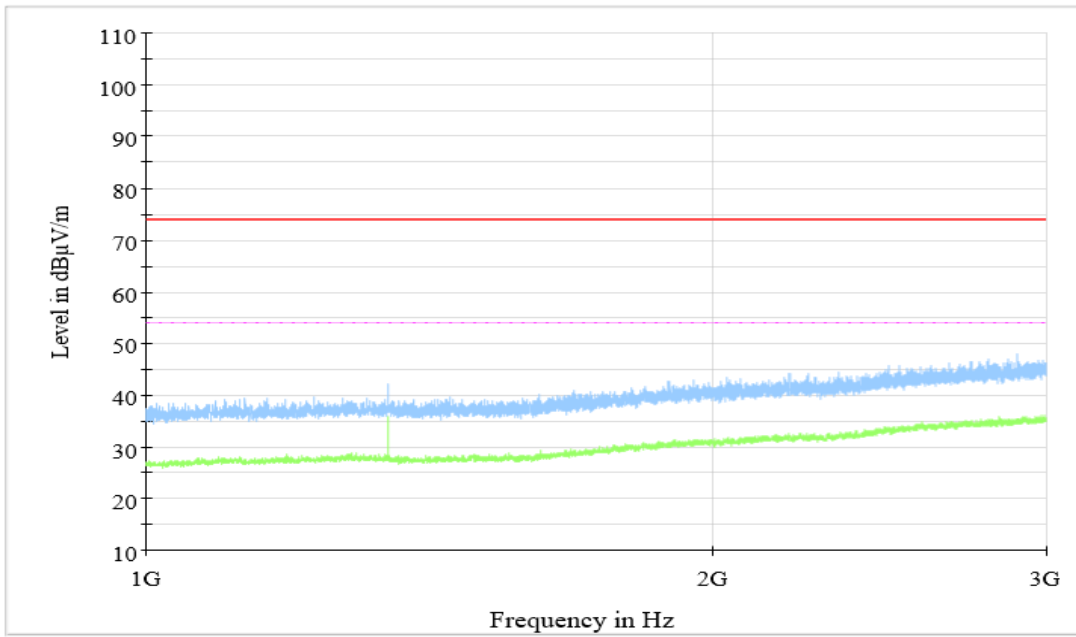
Figure A.1.35. Radiated Emission (Data Transfer : TF Card to PC,1GHz to 3GHz)
