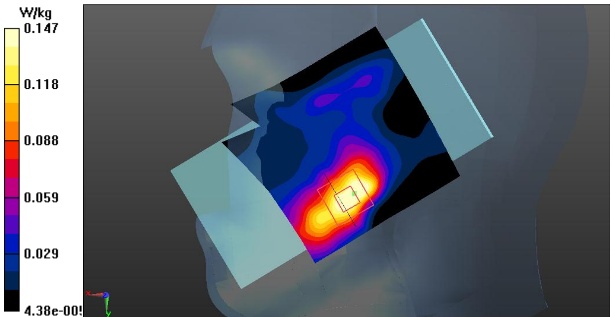
Fig.11 LTE Band 7 Head
