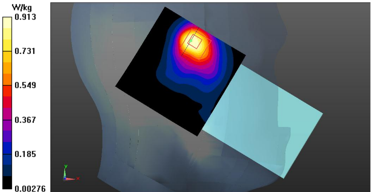
Fig.15 WLAN 2.4G Head
