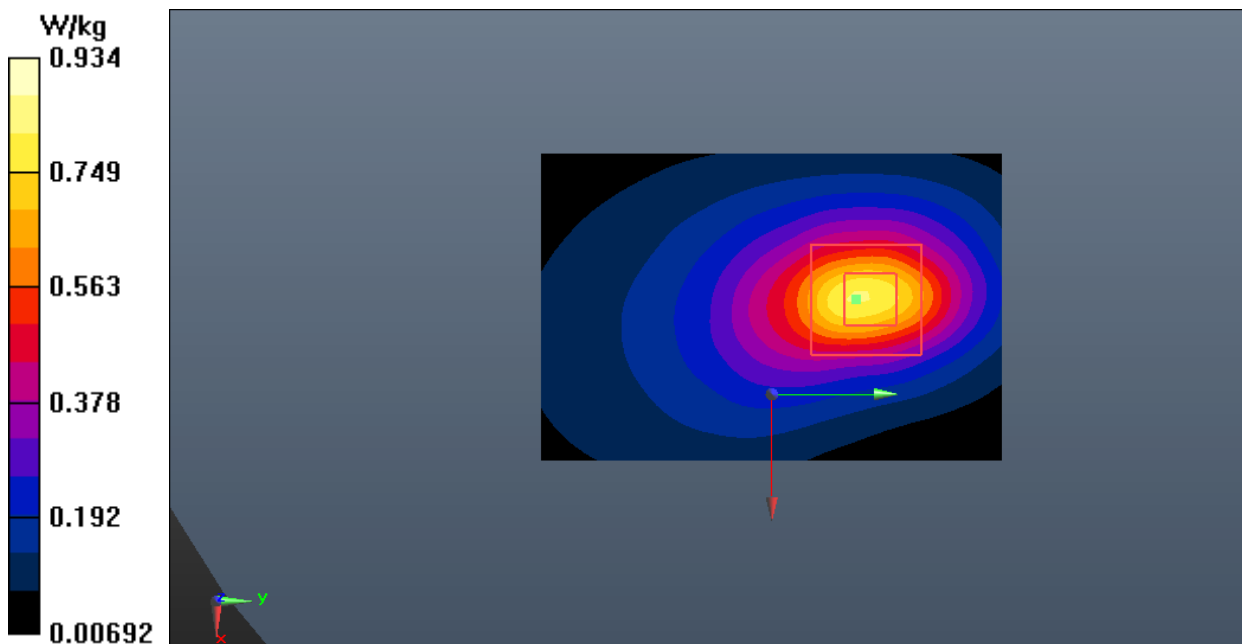
Fig.12 LTE Band 7 Body
