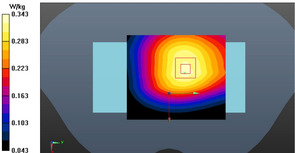
Fig.8 WCDMA Band 5 Body
