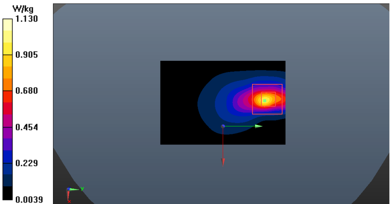
Fig.14 LTE Band 41 Body
