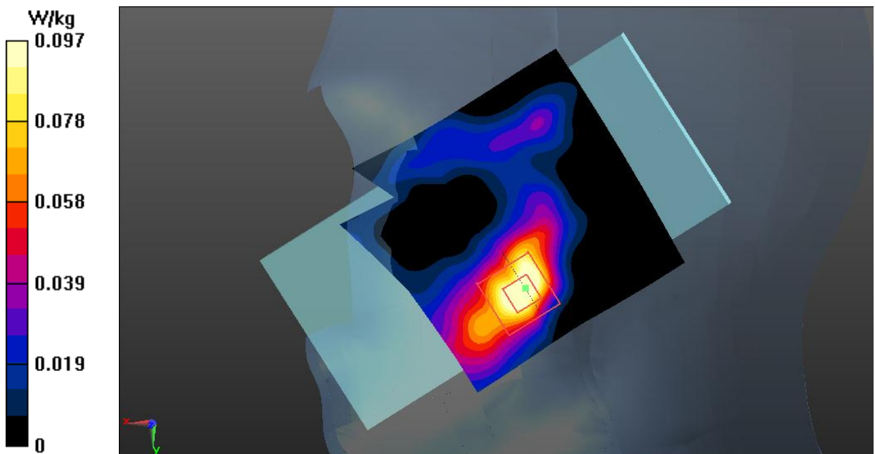
Fig.13 LTE Band 41 Head
