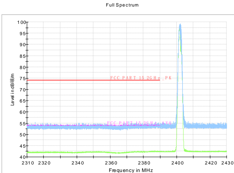
Fig.15. Frequency Band Edges: \pi/4 DQPSK, Channel 0, 2.31 GHz - 2.43GHz
