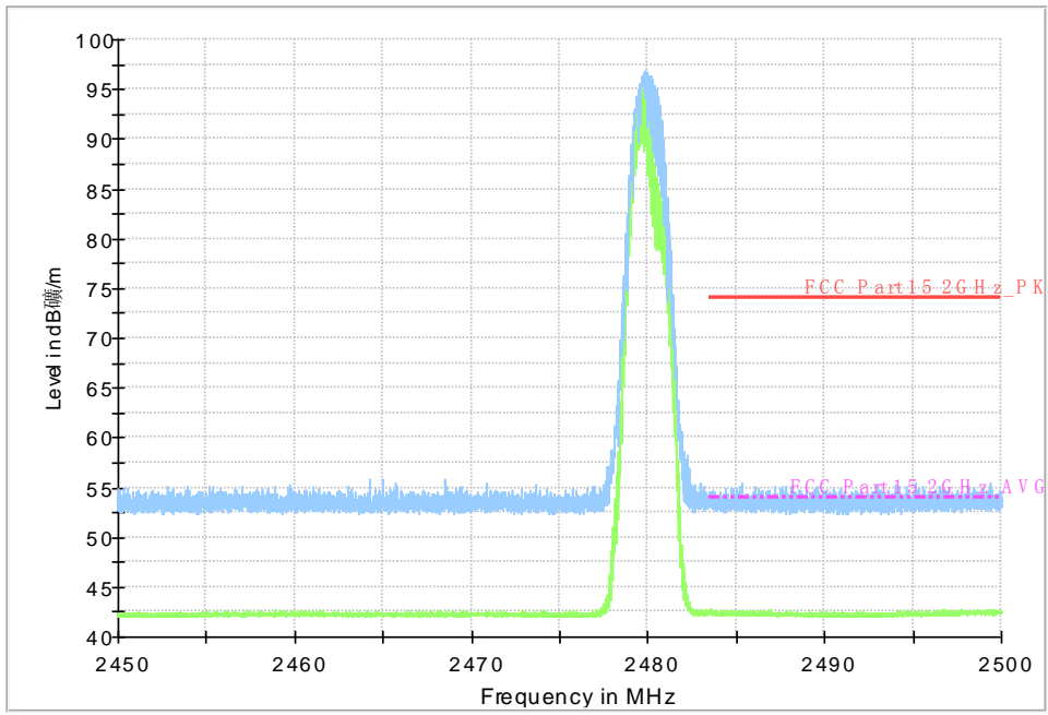
Fig.18. Frequency Band Edges: 8DPSK, Channel 78, 2.45 GHz - 2.50GHz
