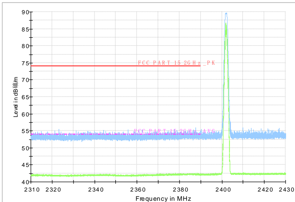
Fig.3. Frequency Band Edges: GFSK, 2402 MHz, 2.31 GHz – 2.43GHz
