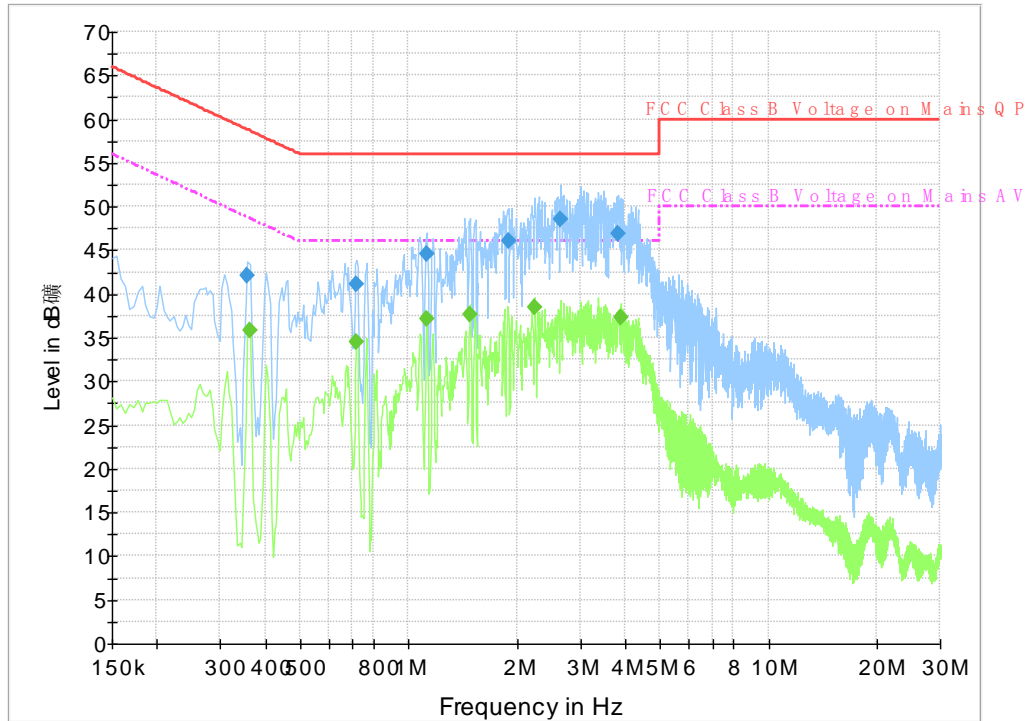
Fig.B.9.1 AC Powerline Conducted Emission- bluetooth
