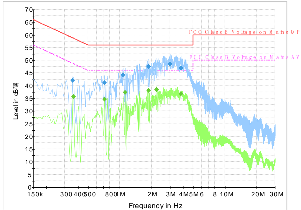
Fig.B.9.2 AC Powerline Conducted Emission-Idle
