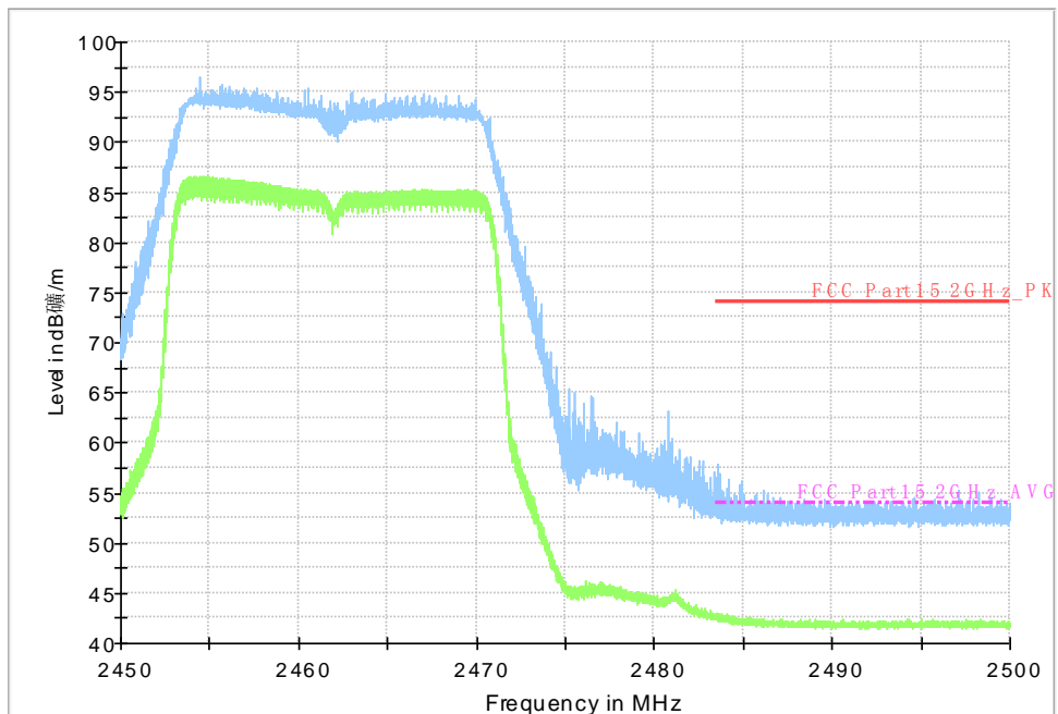
Fig.A.6.2.2 Transmitter Spurious Emission - Radiated (Power): 802.11n-HT20, ch11, 2.45 GHz - 2.50GHz
