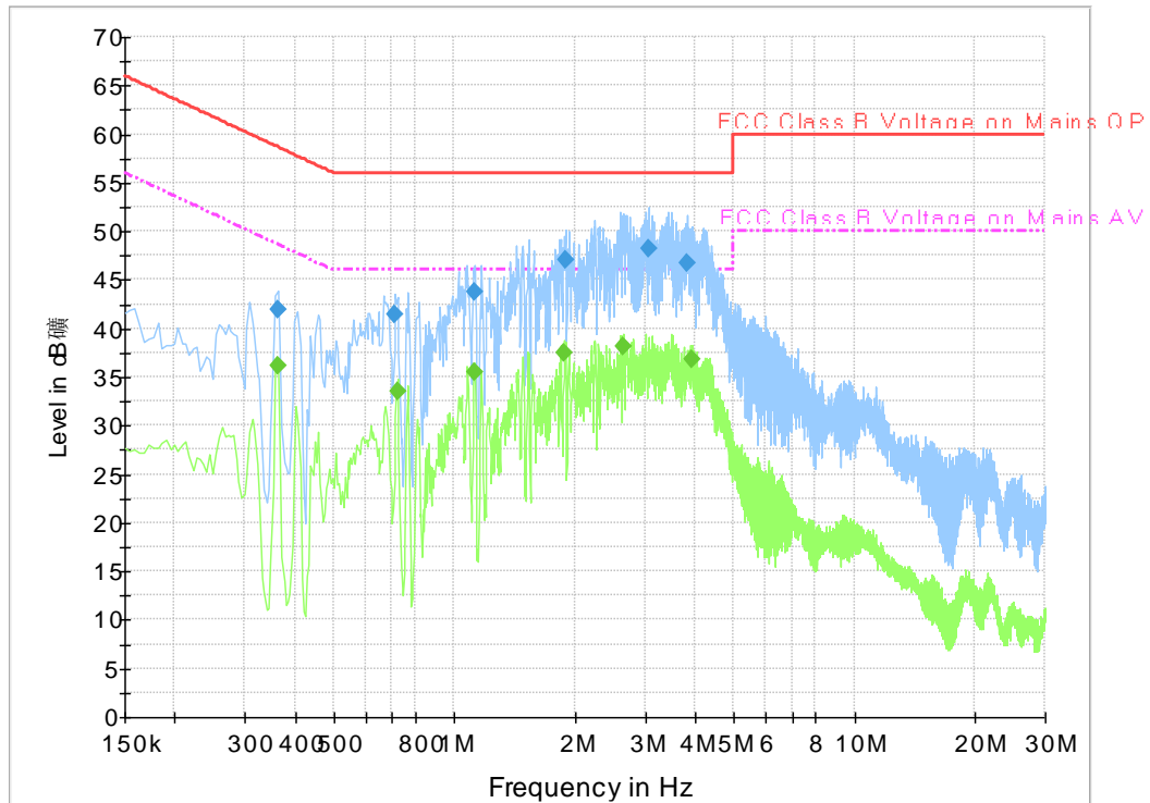
Fig.A.7.1 AC Powerline Conducted Emission-802.11b
