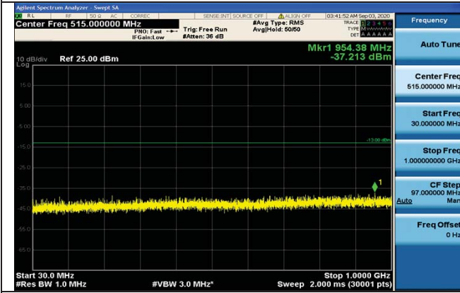
30MHz~1GHz
