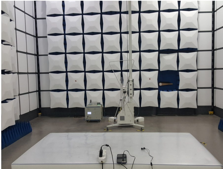
LTE Band2/4/5/7 test photos
