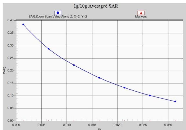
Fig. 1-26 Z-Scan at power reference point (LTEB28)
