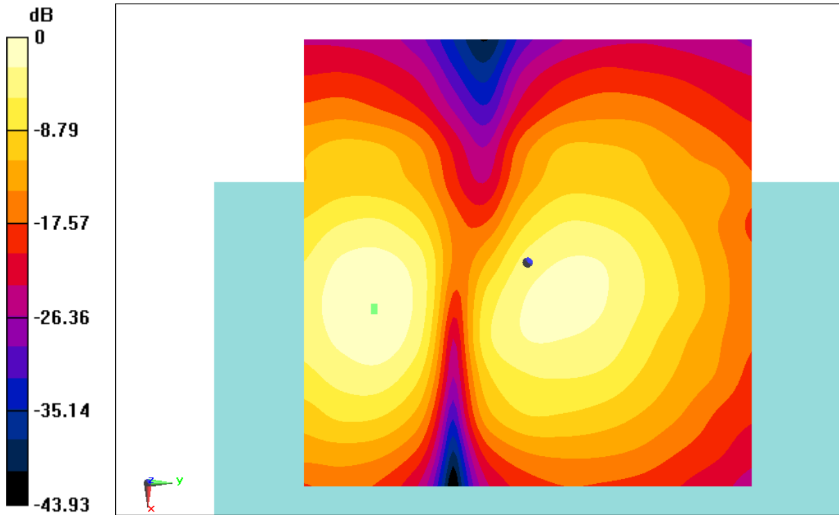
Fig B.5 T-Coil LTE B12
