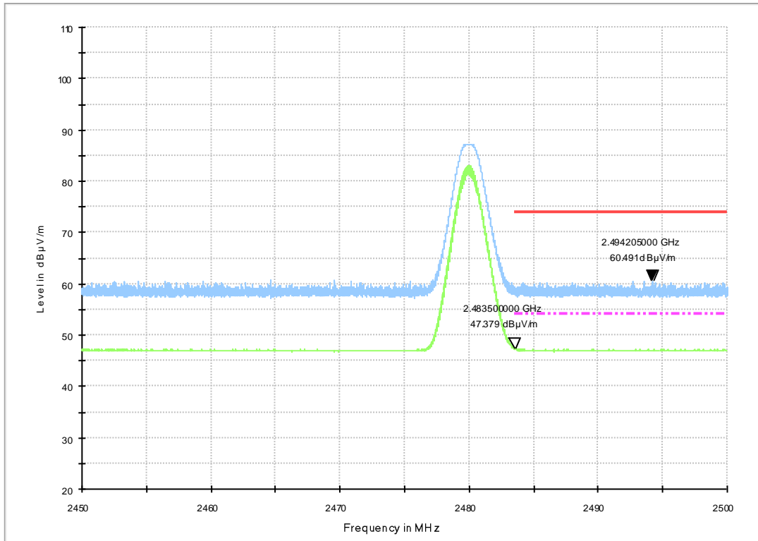
Fig.4. Frequency Band Edges: GFSK, 2480 MHz, 2.45 GHz - 2.50GHz
