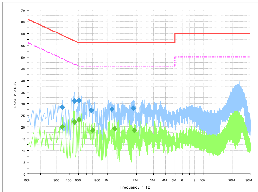
Fig.B.9.1 AC Powerline Conducted Emission-traffic
