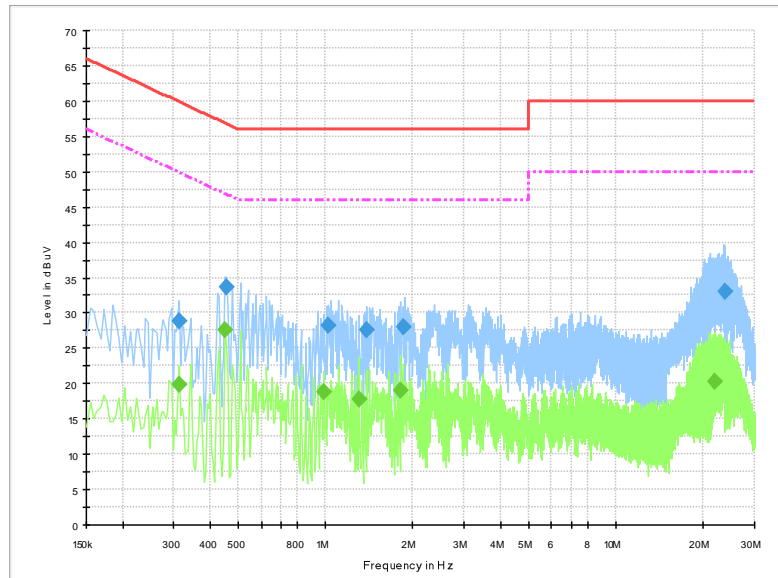
Fig.B.11.1 AC Powerline Conducted Emission-traffic
