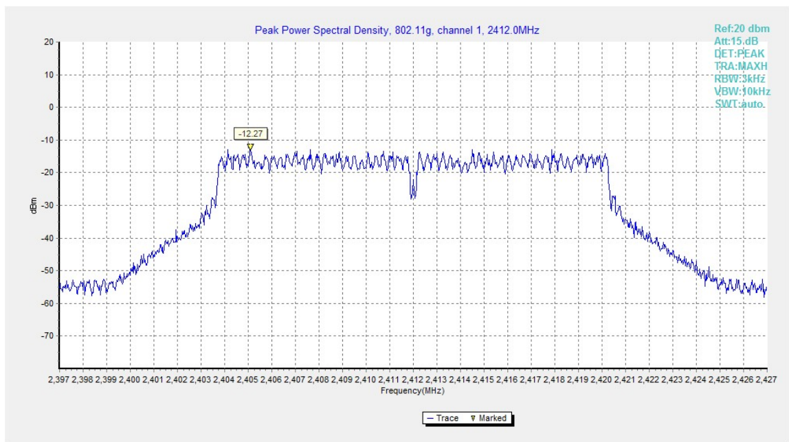
Fig.B.3.4 Power Spectral Density (802.11g, Ch 1)
