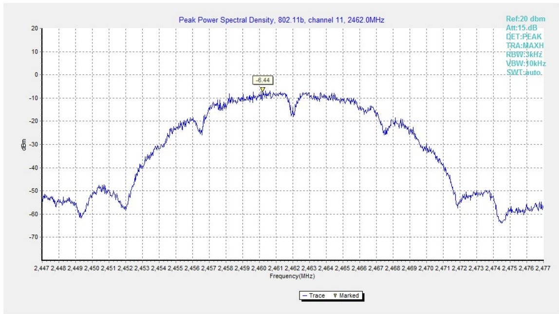
Fig.B.3.3 Power Spectral Density (802.11b, Ch 11)
