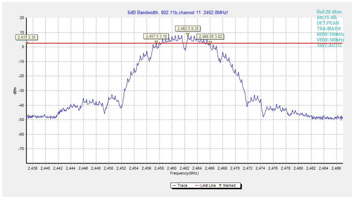
Fig.B.4.3 Occupied 6dB Bandwidth (802.11b, Ch 11)
