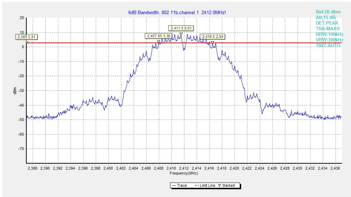
Fig.B.4.1 Occupied 6dB Bandwidth(802.11b,Ch 1)
