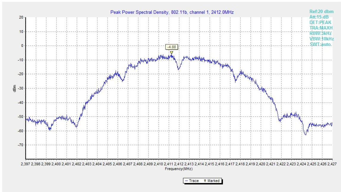
Fig.B.3.1 Power Spectral Density(802.11b,Ch1)
