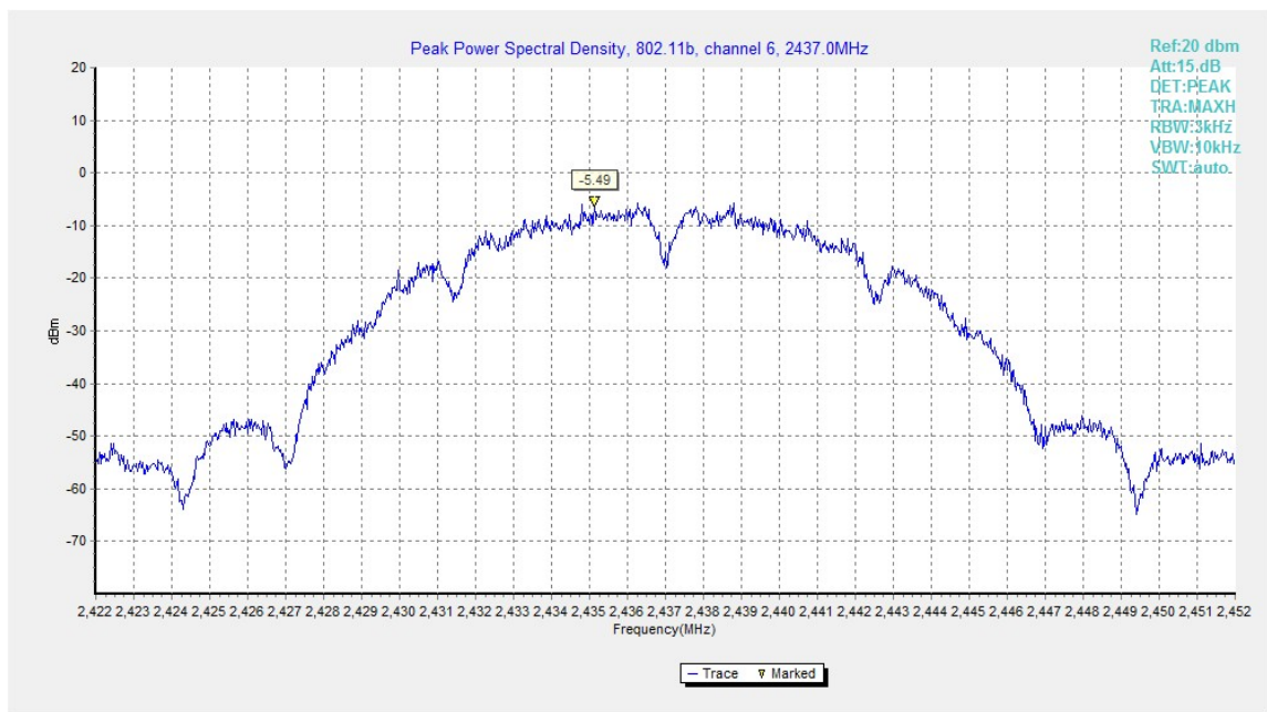
Fig.B.3.2 Power Spectral Density (802.11b, Ch 6)
