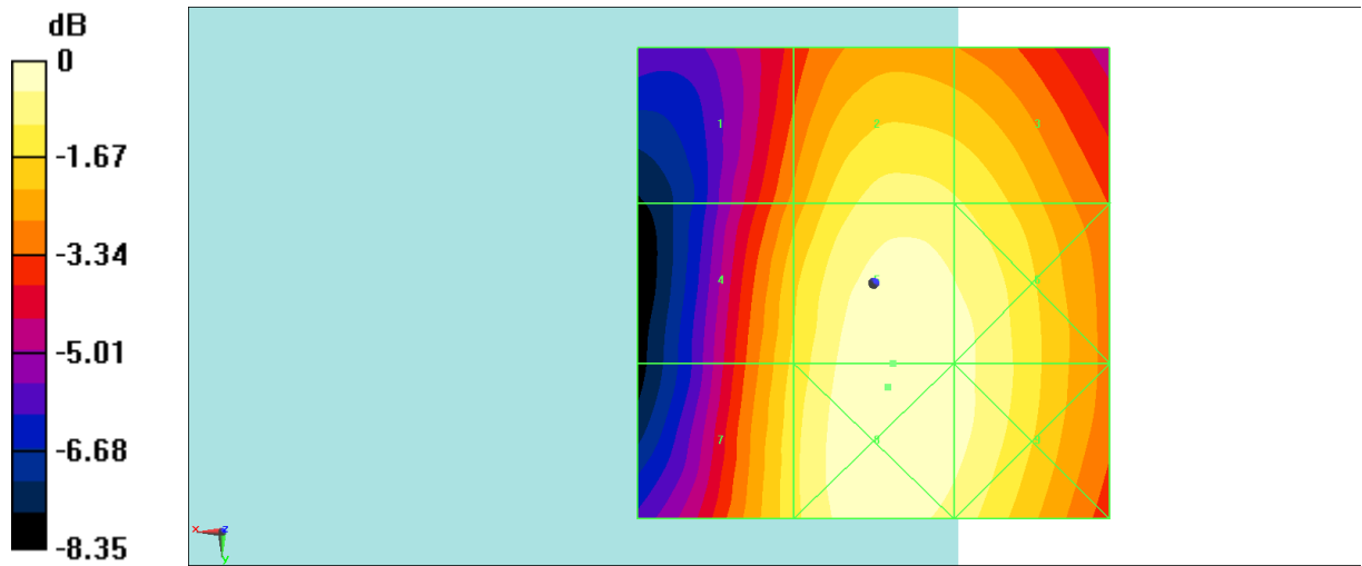
Fig B.2 HAC RF E-Field GSM 1900 Middle
